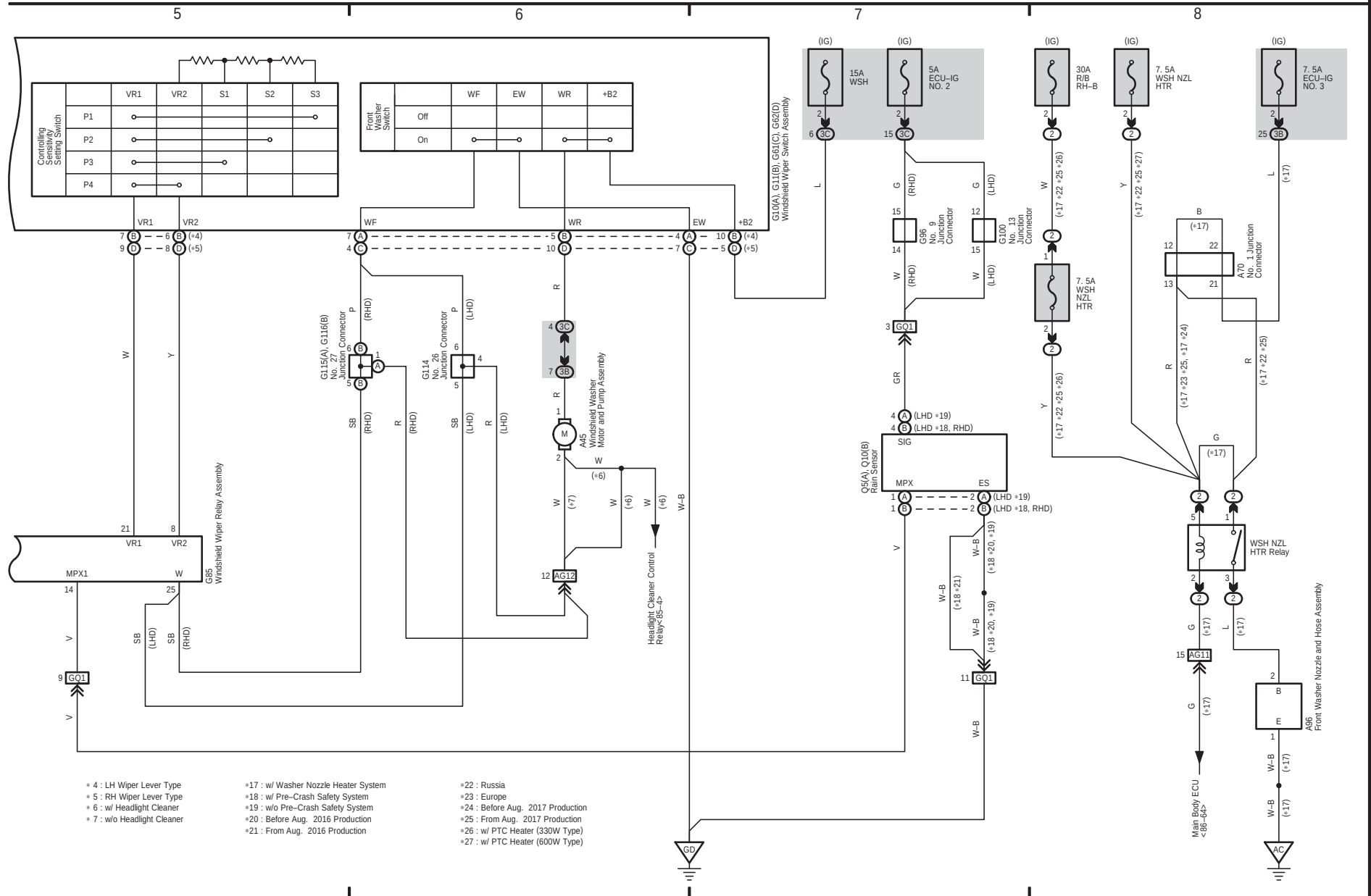
Front Wiper and Washer (w/ Auto Wiper System) (From Oct. 2015 Production)
