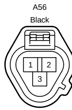
90980-11016 (Headlight Leveling Motor)
