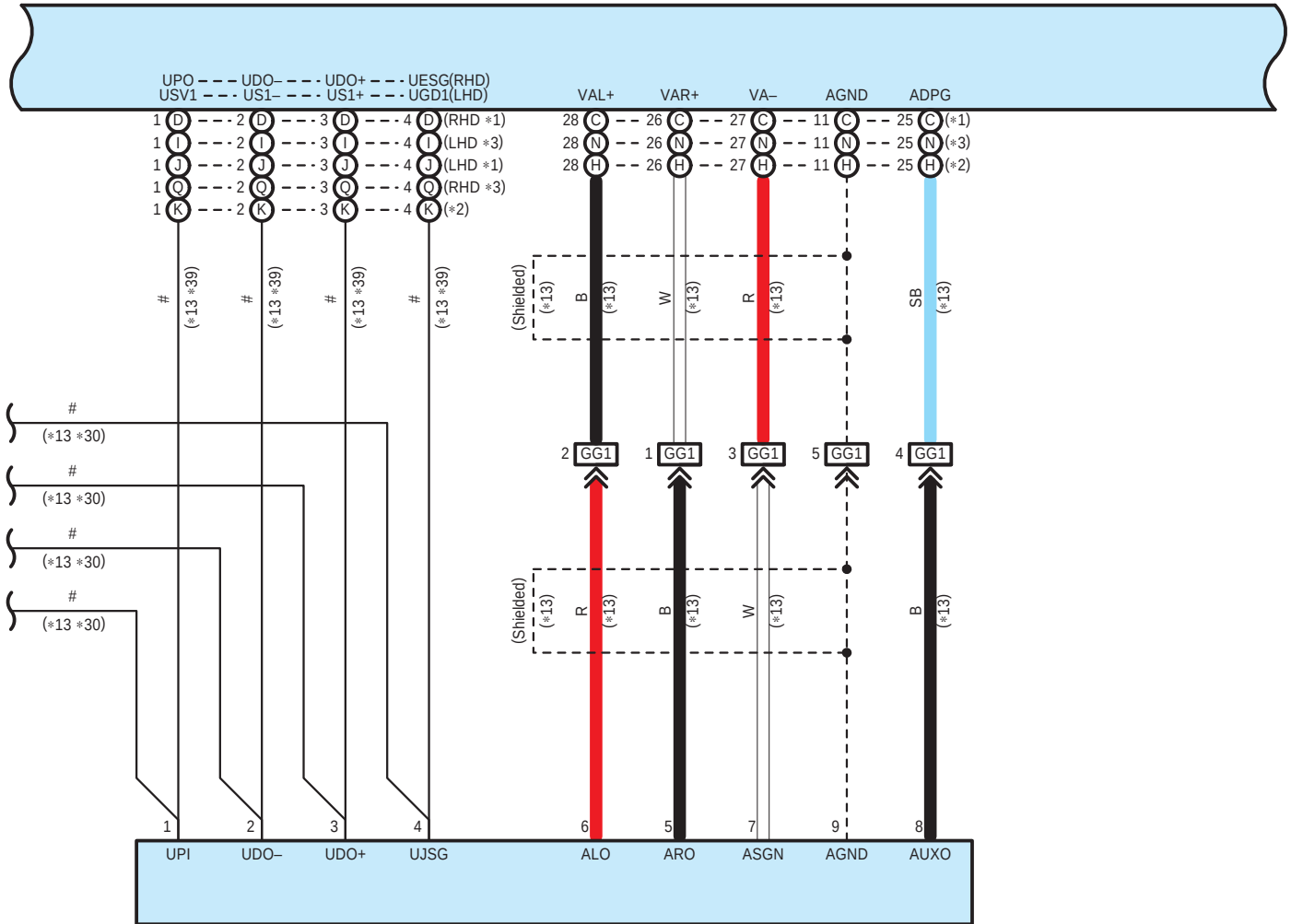
G145 No. 1 Stereo Jack Adapter Assembly
