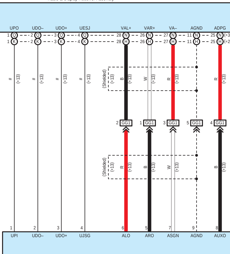
G145 No. 1 Stereo Jack Adapter Assembly
