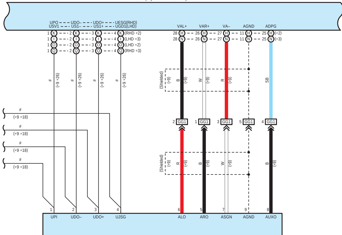
G145 No. 1 Stereo Jack Adapter Assembly
