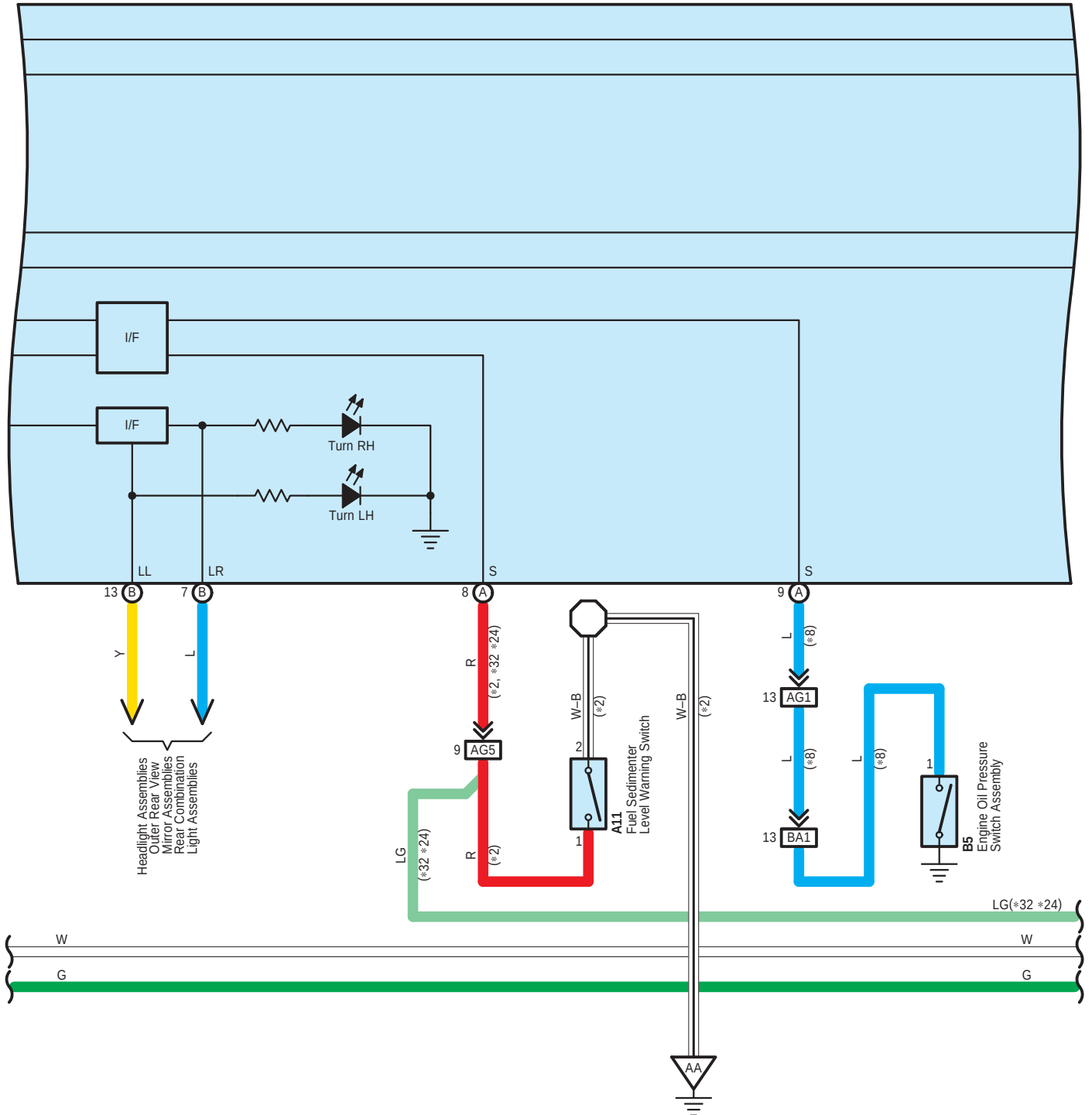
G16(A), G17(B) Combination Meter Assembly
