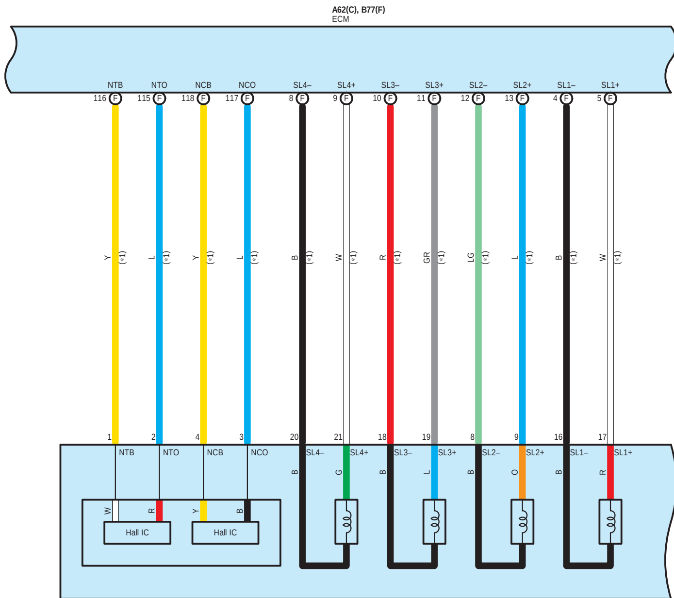
B78 ECT Solenoid (Transmission Wire)
