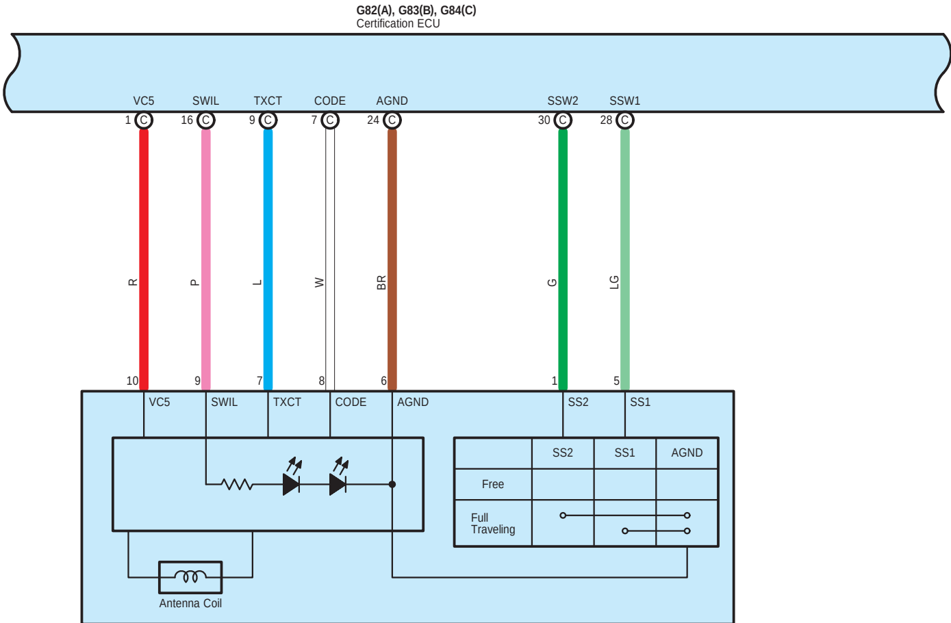
G24 Engine Switch
