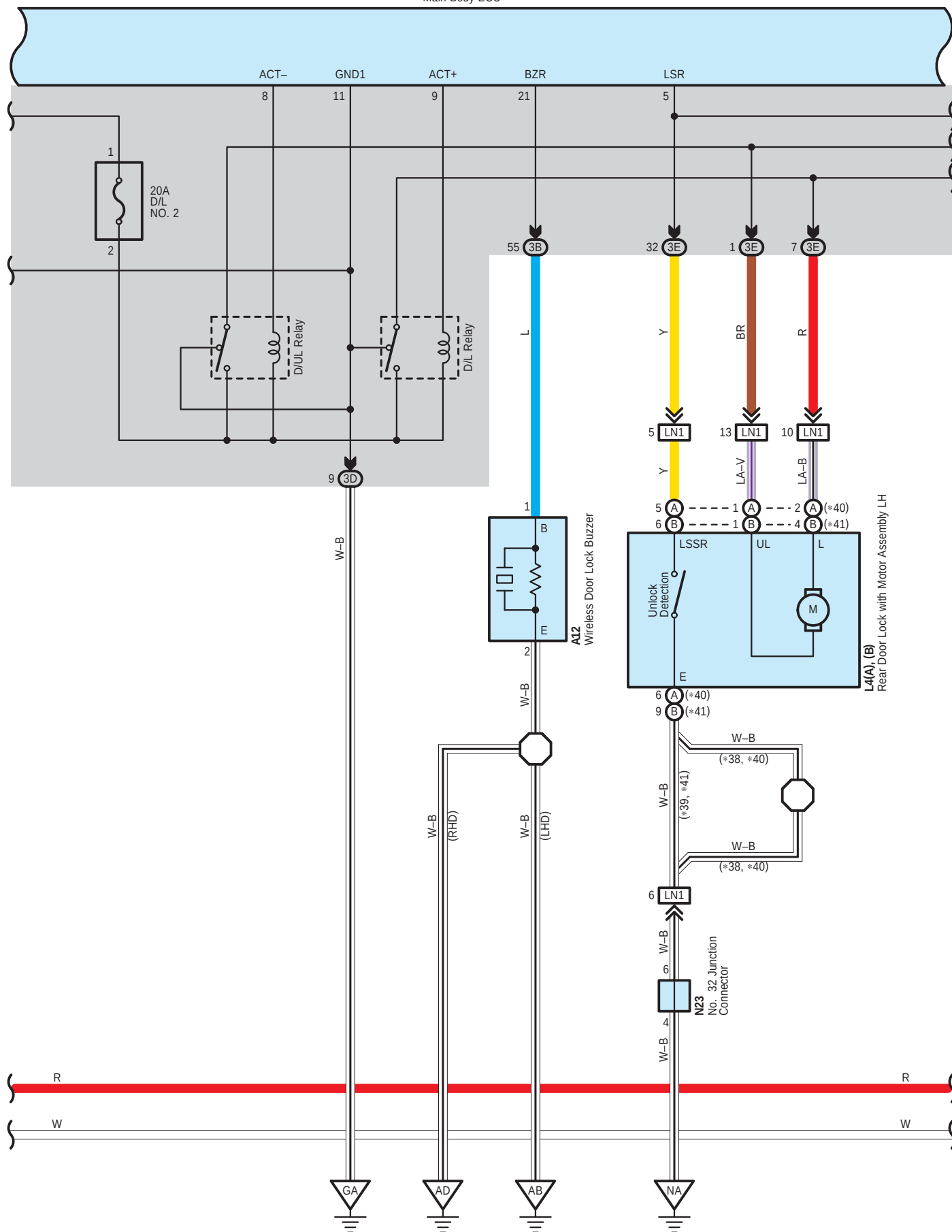
G78(A), G79(B), G202(C) Main Body ECU
