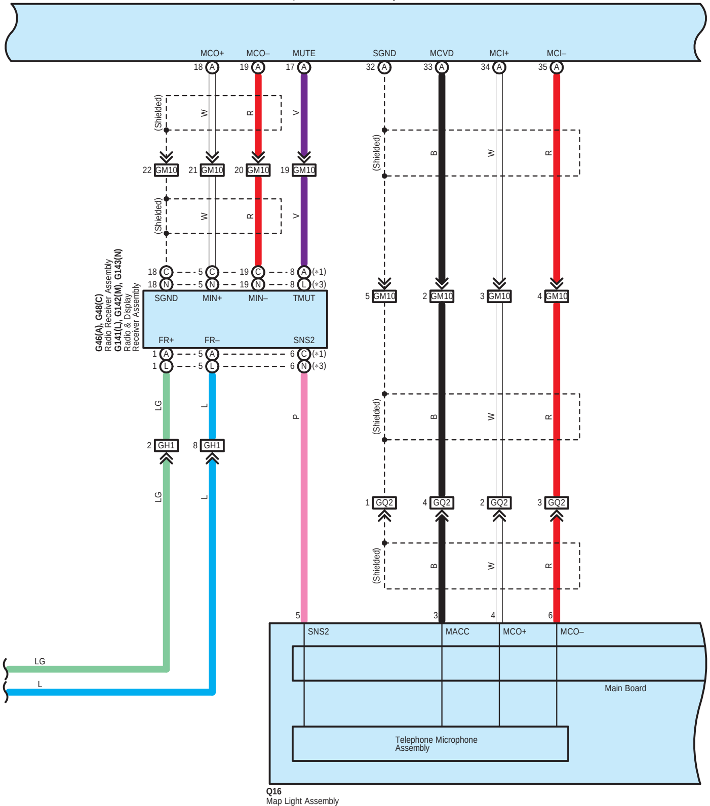
M38(A), M42(B), M43(C) Telephone Transceiver Assembly
