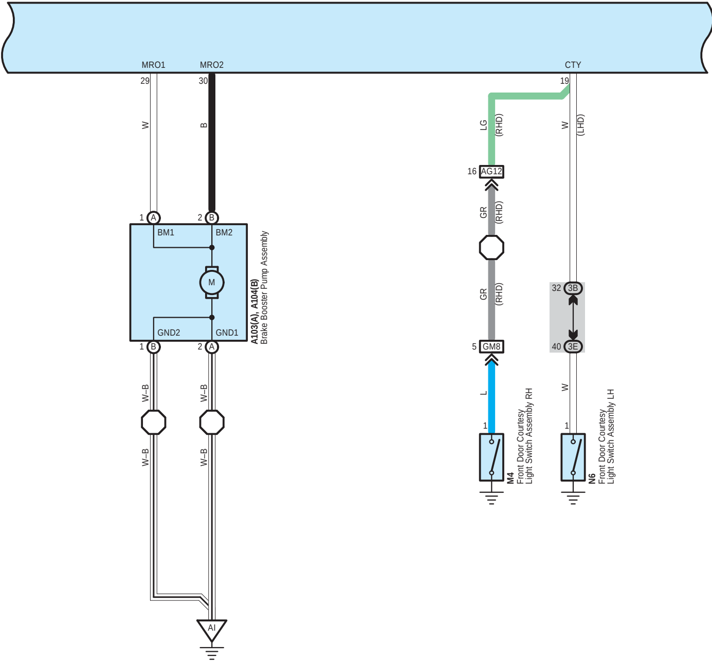
A110 Brake Booster with Master Cylinder Assembly
