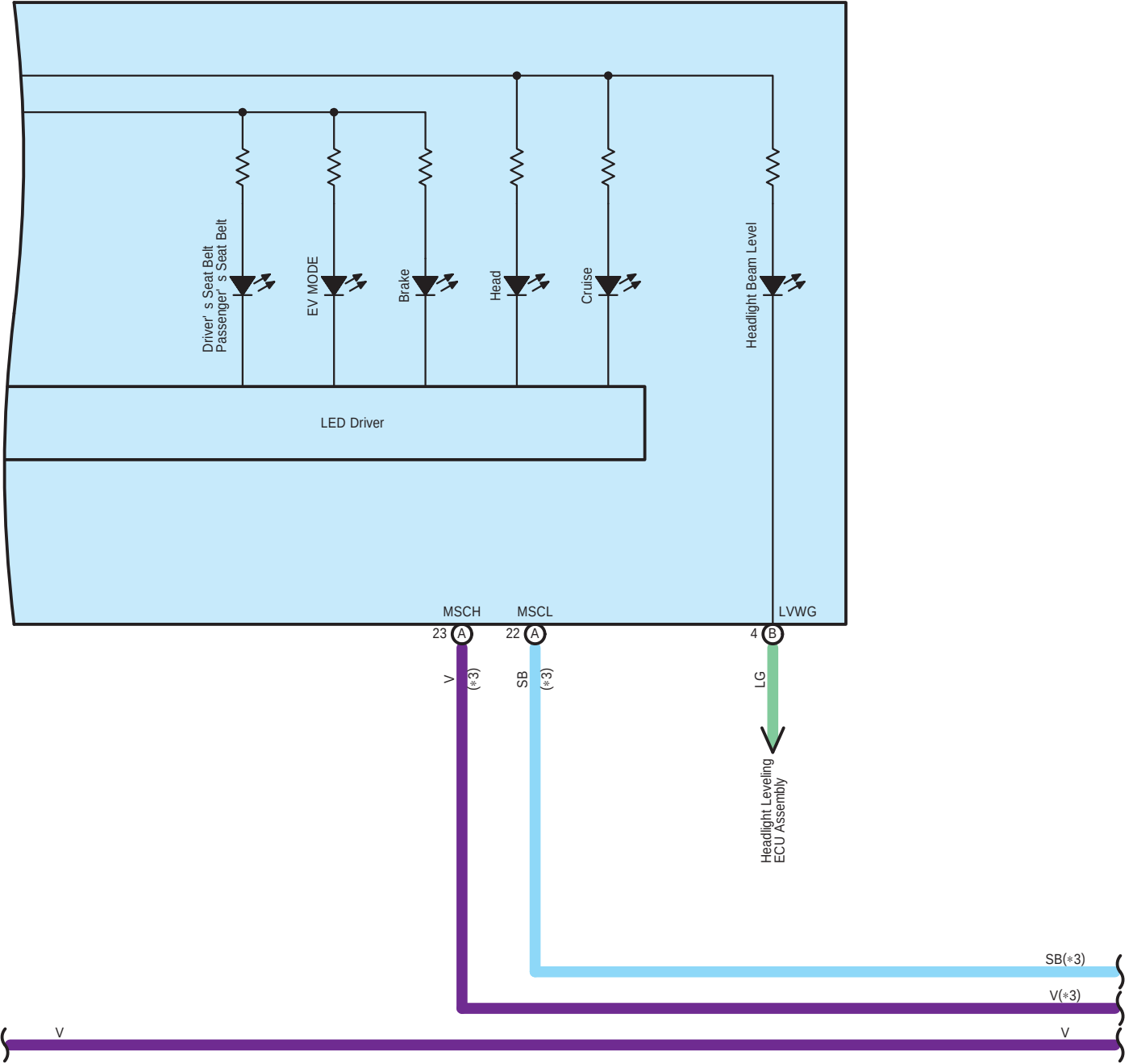
G16(A), G17(B) Combination Meter Assembly
