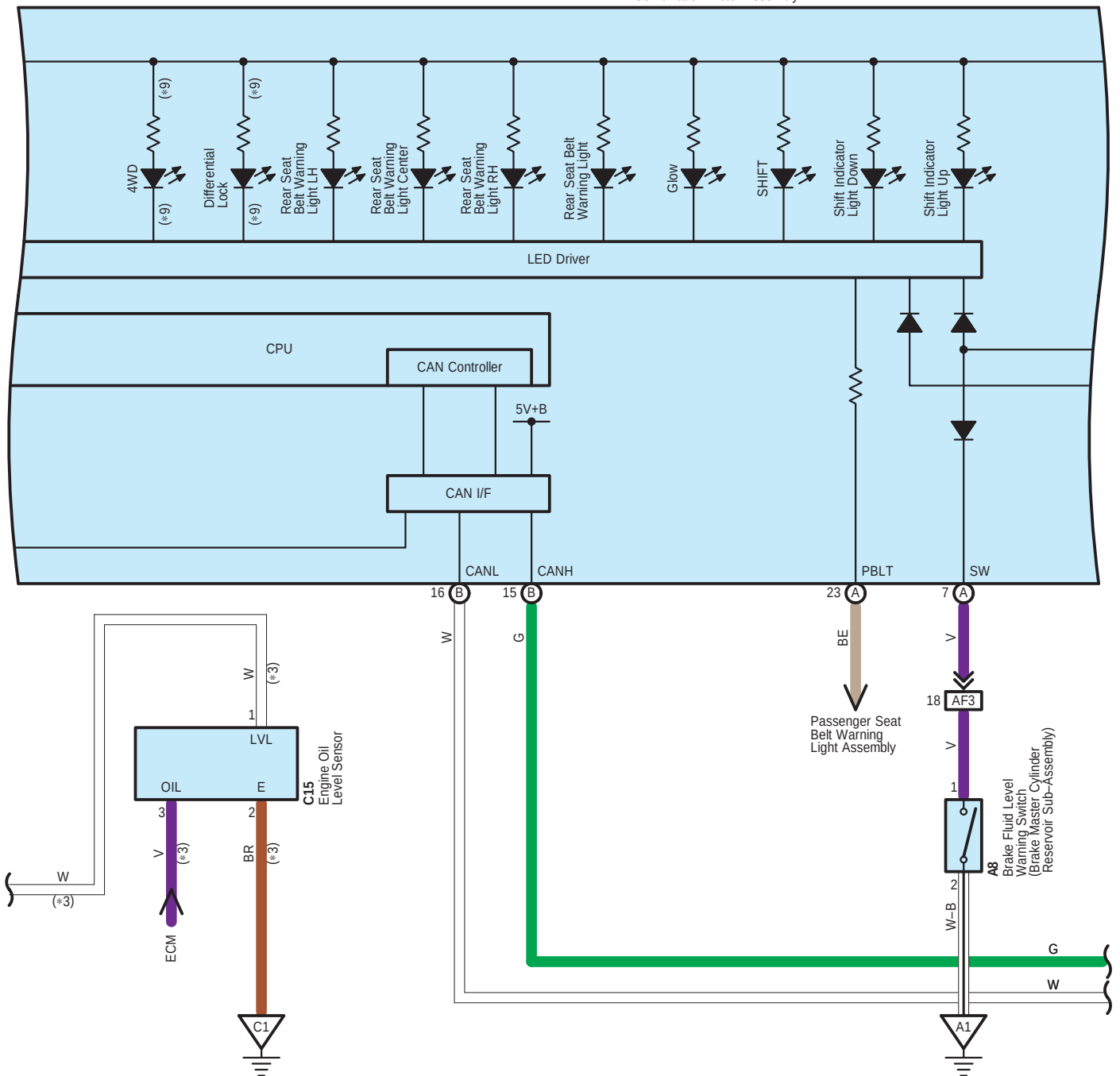
F1(A), F2(B) Combination Meter Assembly
