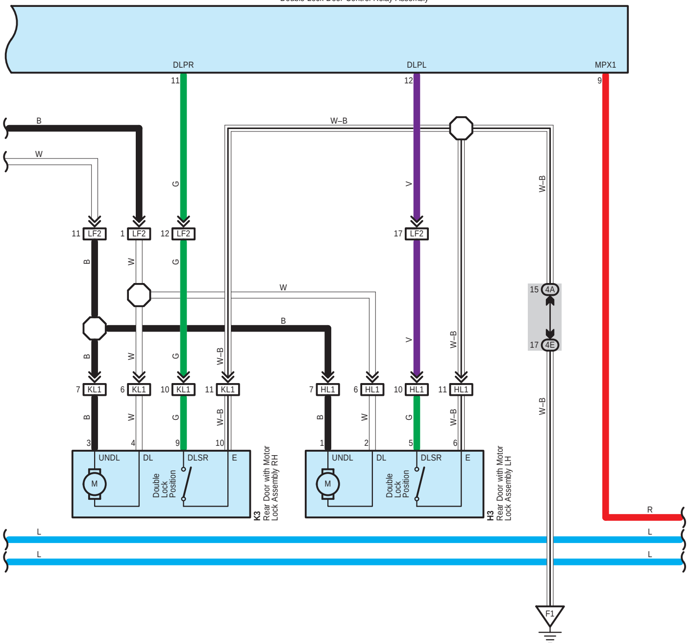
F89 Double Lock Door Control Relay Assembly
