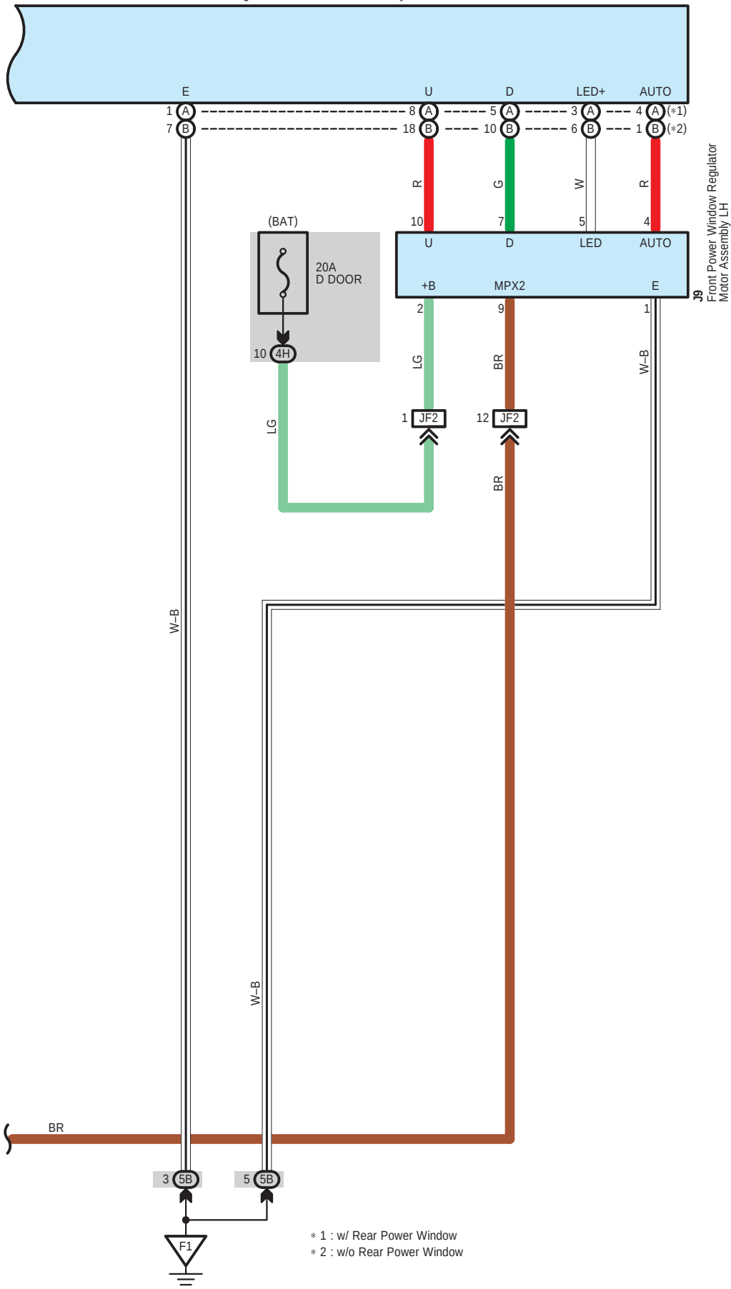
J1(A), (B) Power Window Regulator Master Switch Assembly
