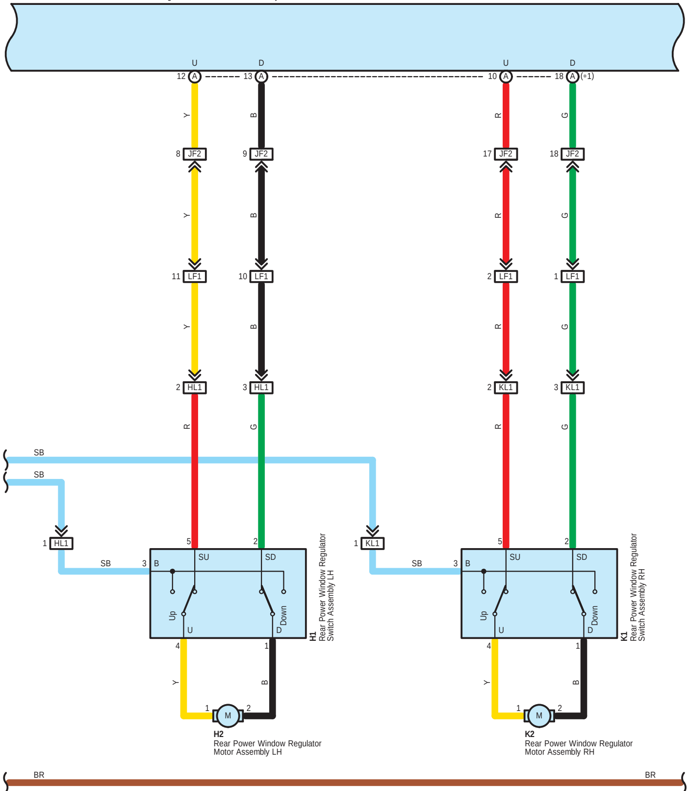
J1(A), (B) Power Window Regulator Master Switch Assembly
