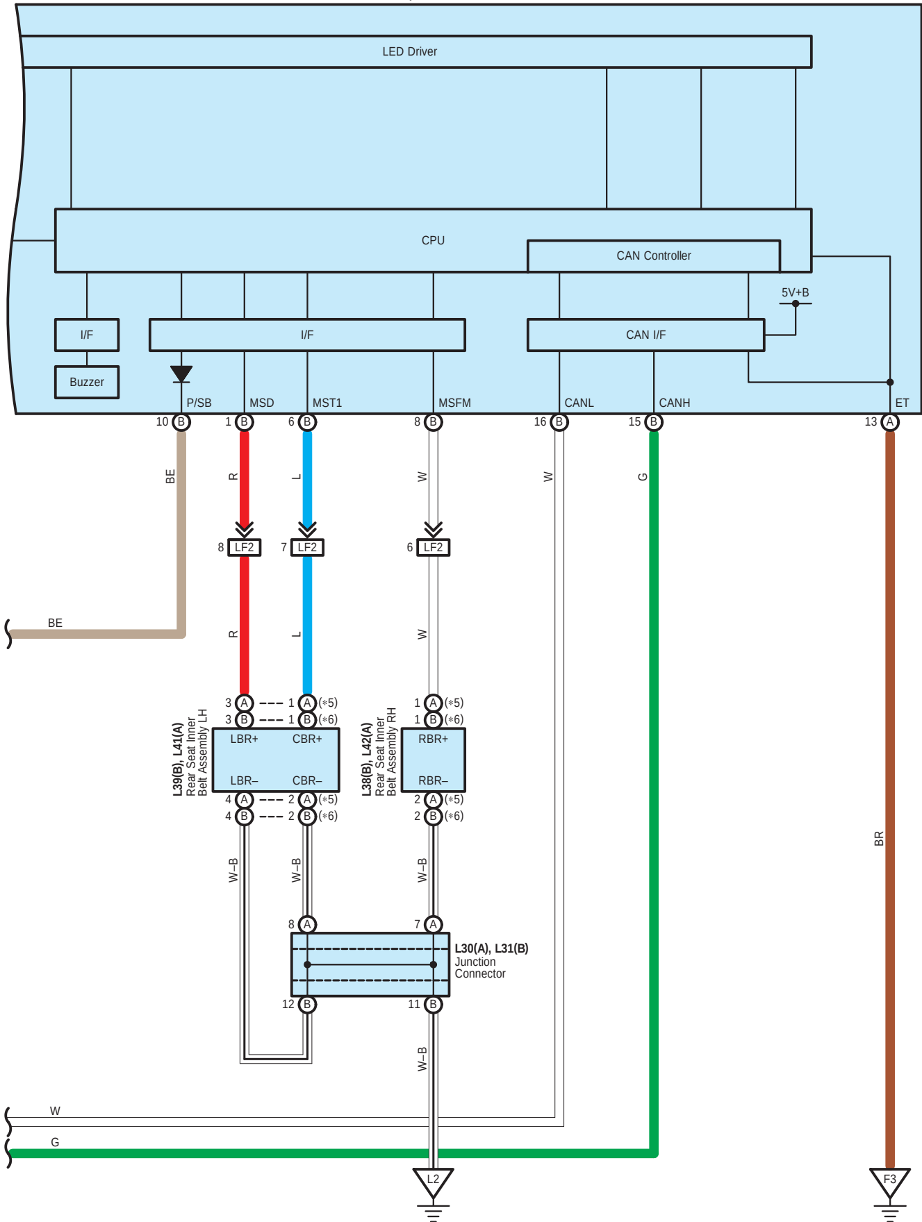
F1(A), F2(B) Combination Meter Assembly
