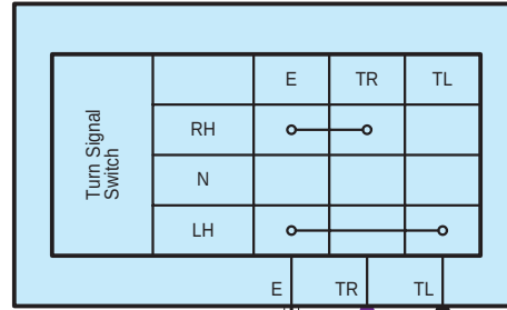
F6 Headlight Dimmer Switch Assembly
