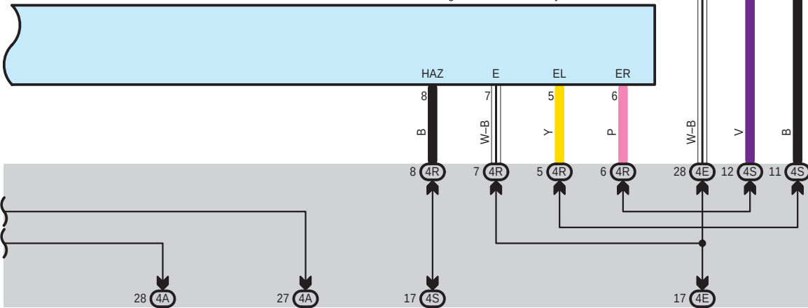
F90 Turn Signal Flasher Assembly
