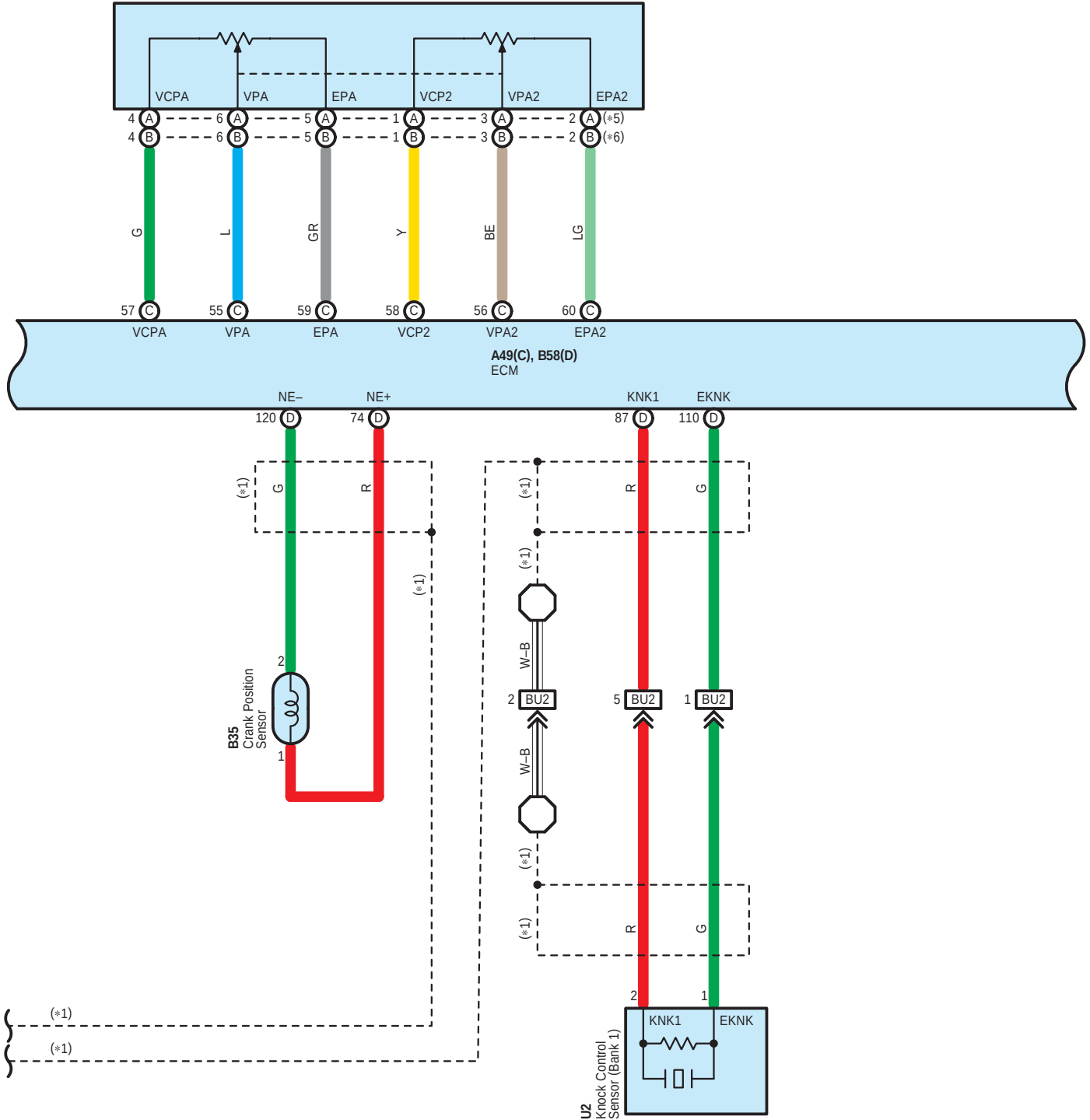
A32(A), A59(B) Accelerator Position Sensor (Accelerator Pedal Assembly)
