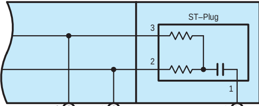
L27(A), L28(B), L29(C), L30(D) Junction Connector
