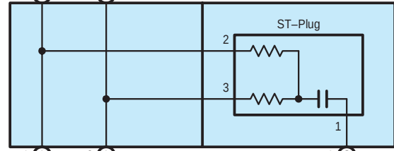
D69(A), D70(B), D71(C) Junction Connector
