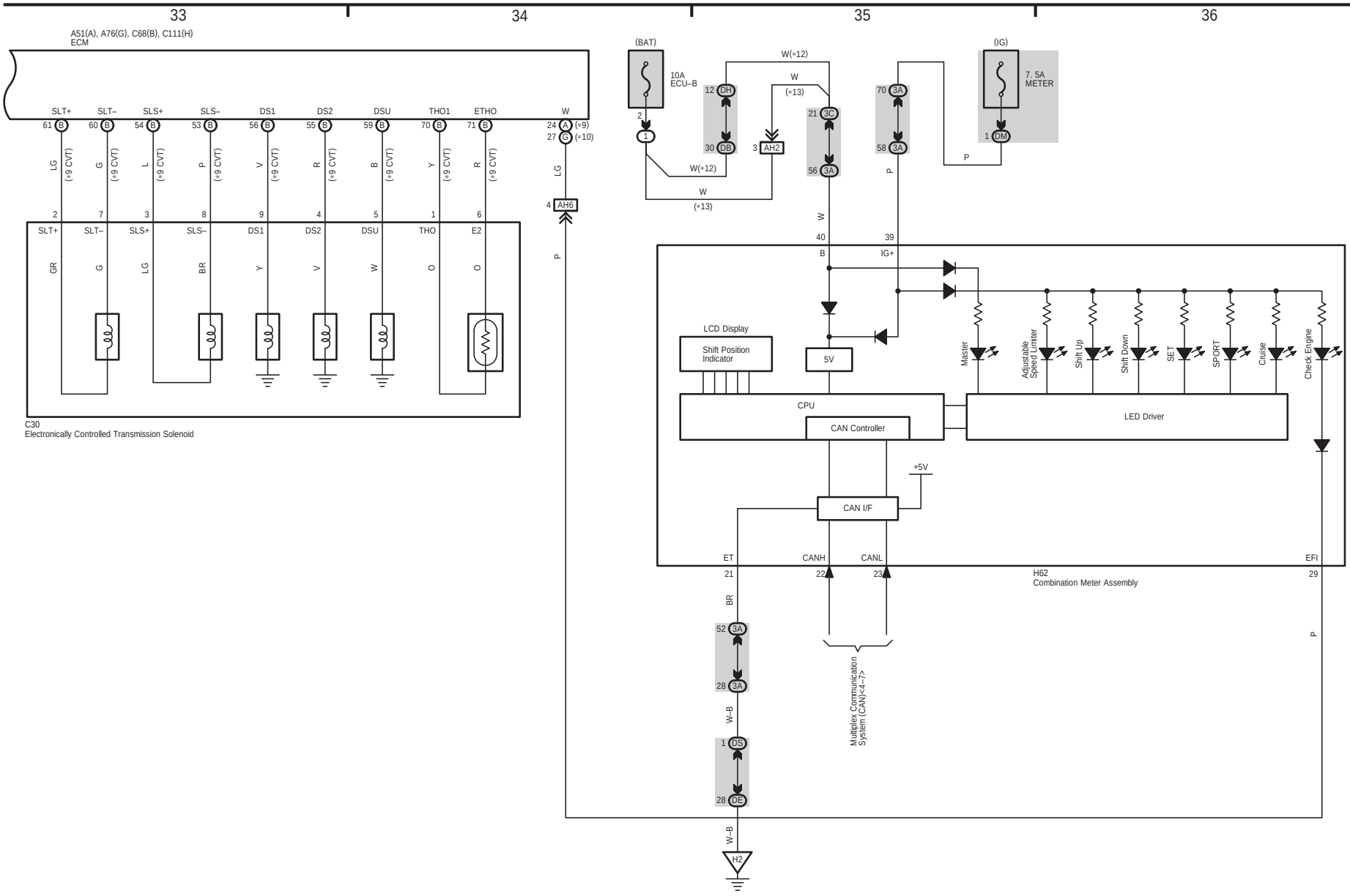
CVT and Shift Indicator (2ZR-FAE)
