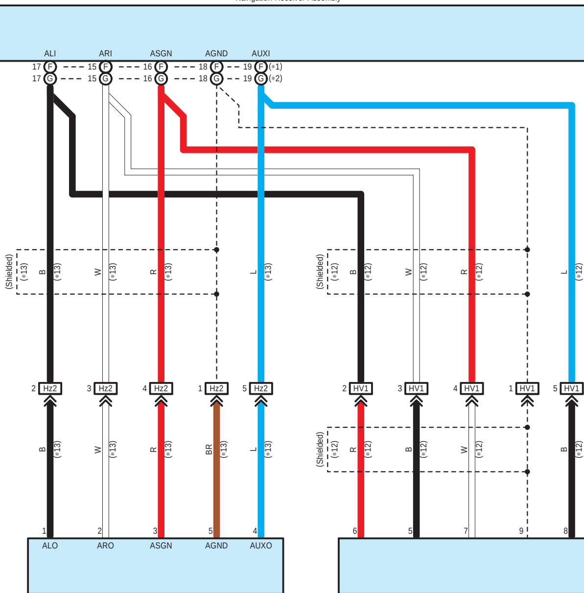
z6 No. 1 Stereo Jack Adapter Assembly
