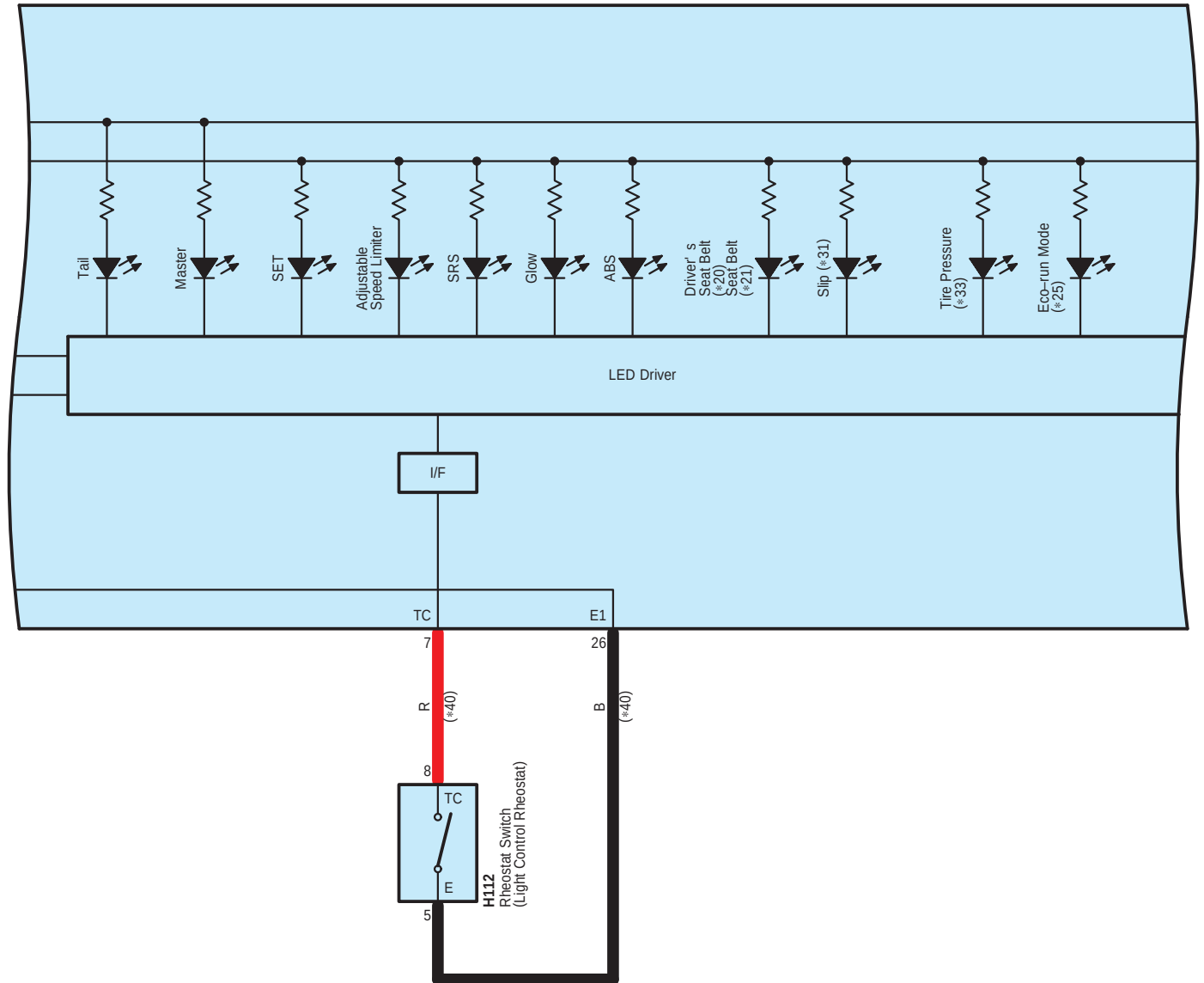
H62 Combination Meter Assembly
