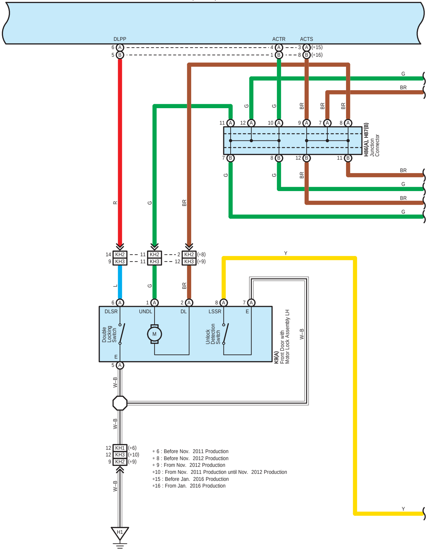
H50(A), H135(B) Double Lock Door Control Relay Assembly
