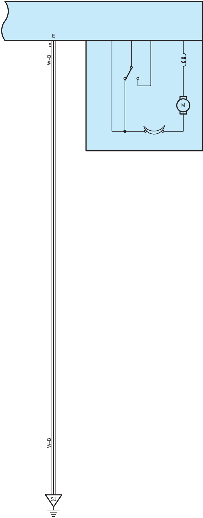
S3 Rear Wiper Motor Assembly
