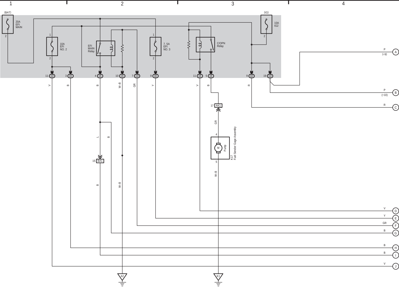
CVT and Shift Indicator and Engine Control (1NZ-FE) (From Aug. 2012 Production)
