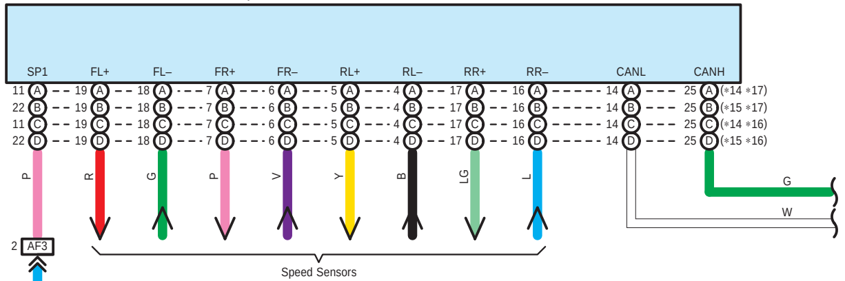
A54(A), A55(B), A56(C), A57(D) Skid Control ECU with Actuator Assembly
