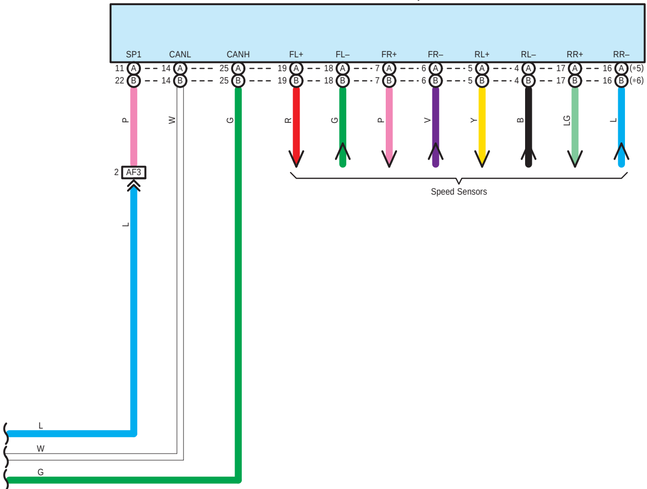
A54(A), A55(B) Skid Control ECU with Actuator Assembly
