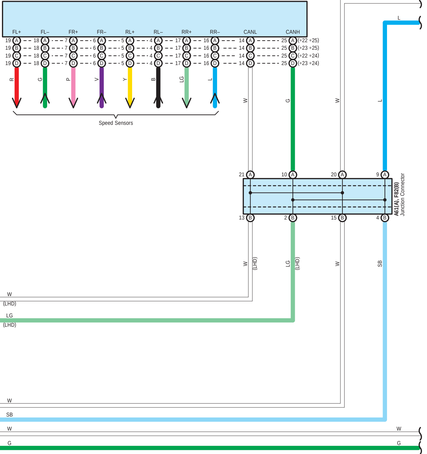
A54(A), A55(B), A56(C), A57(D) Skid Control ECU with Actuator Assembly
