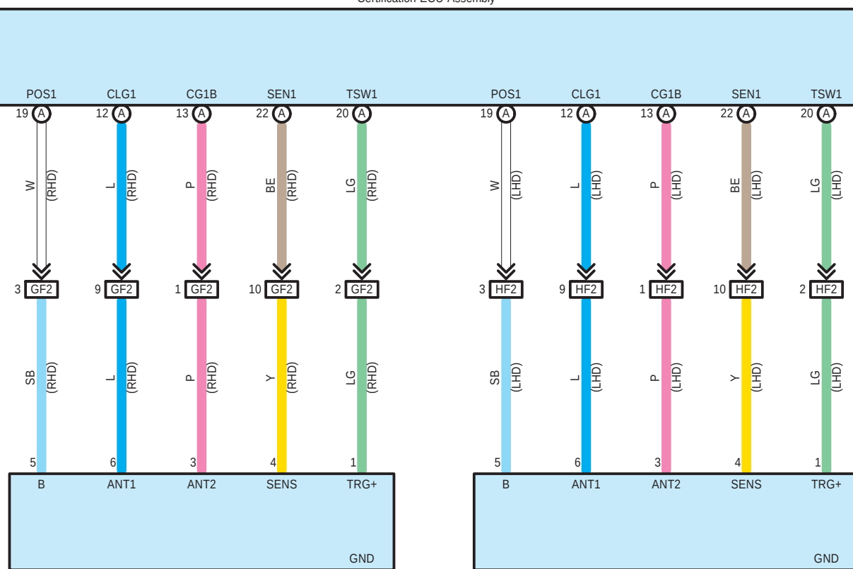
G10 Electrical Key Antenna RH
