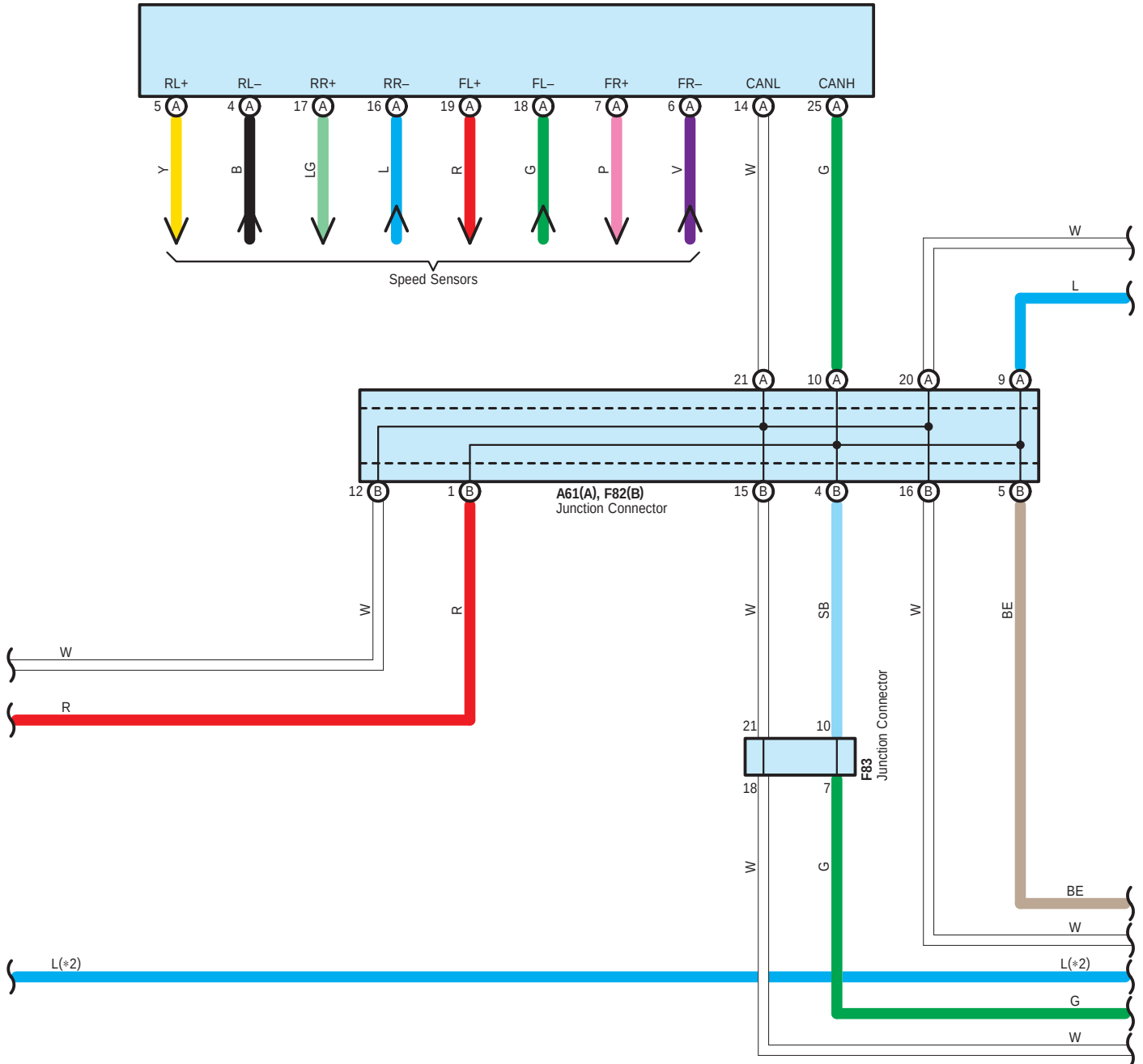
A54(A) Skid Control ECU with Actuator Assembly
