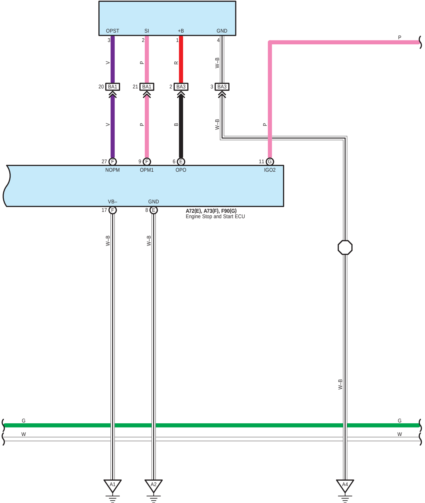
B89 Oil Pump Motor Assembly
