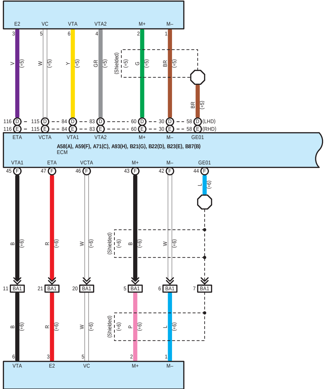
B29 Throttle with Motor Body Assembly
