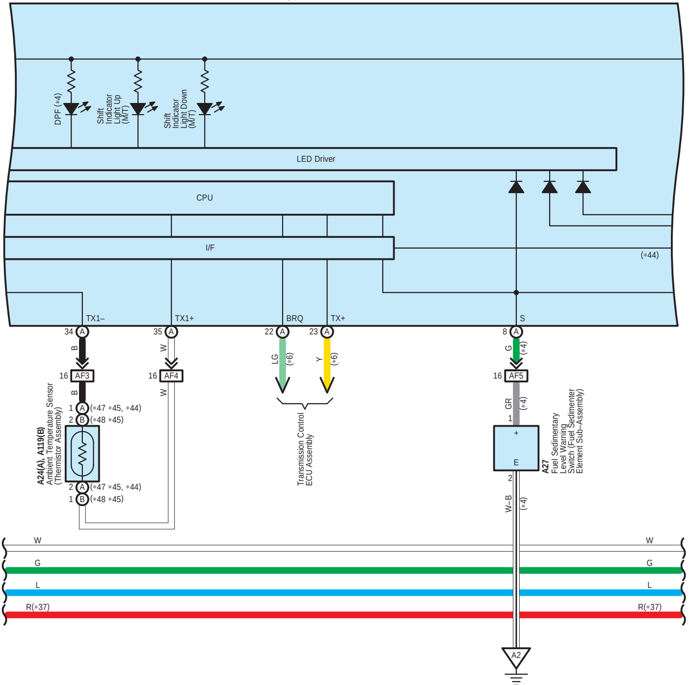
F1(A), F3(B) Combination Meter Assembly
