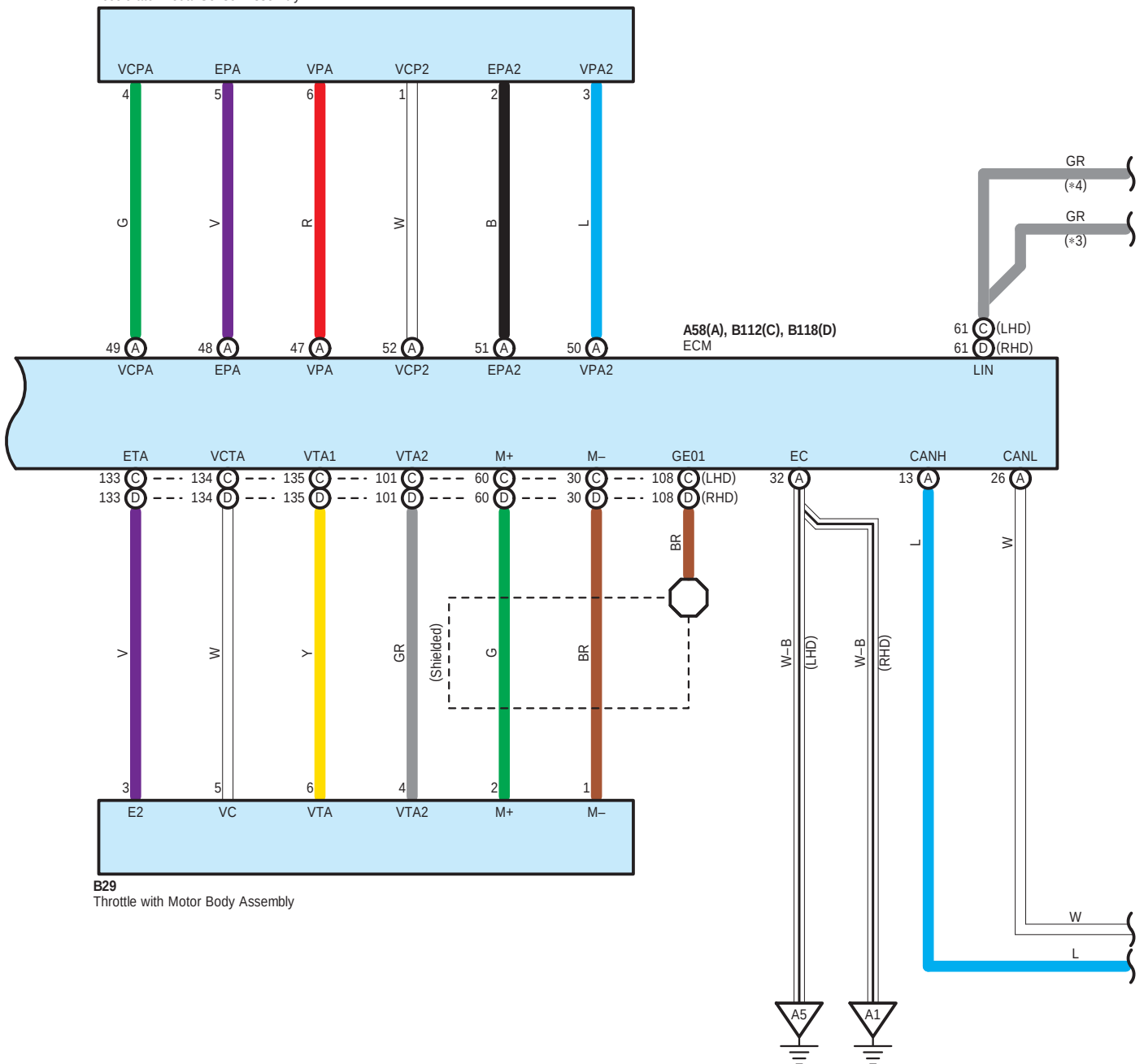
A36 Accelerator Pedal Sensor Assembly
