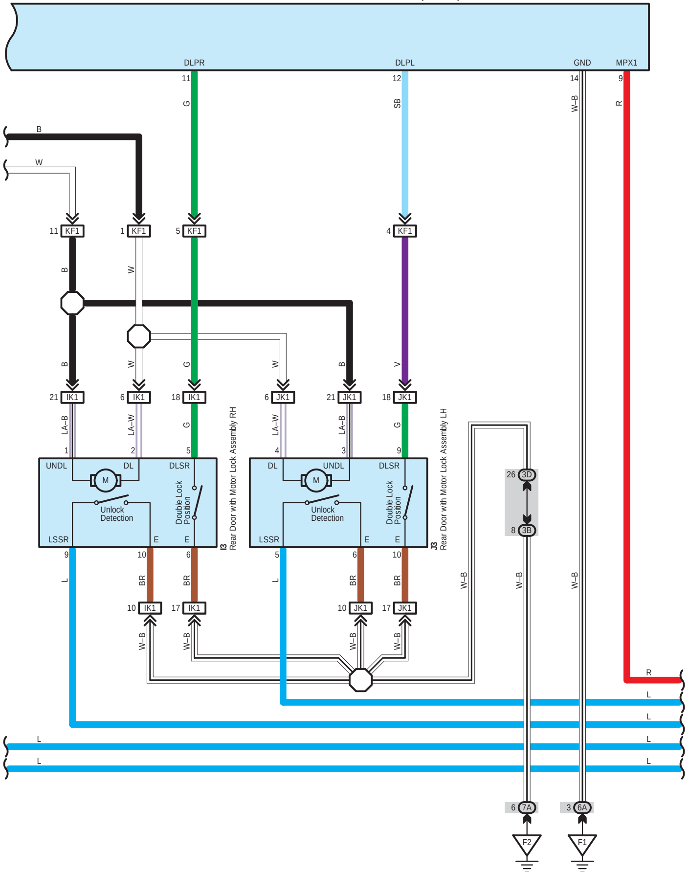
F79 Double Lock Door Control Relay Assembly
