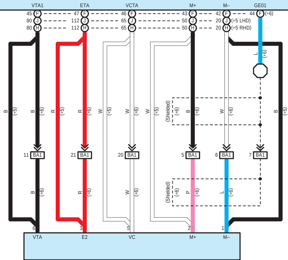
B29 Throttle with Motor Body Assembly
