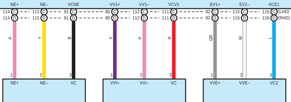
B24 No. 1 Crank Position Sensor
