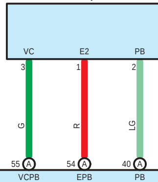
A33 Vacuum Sensor Assembly
