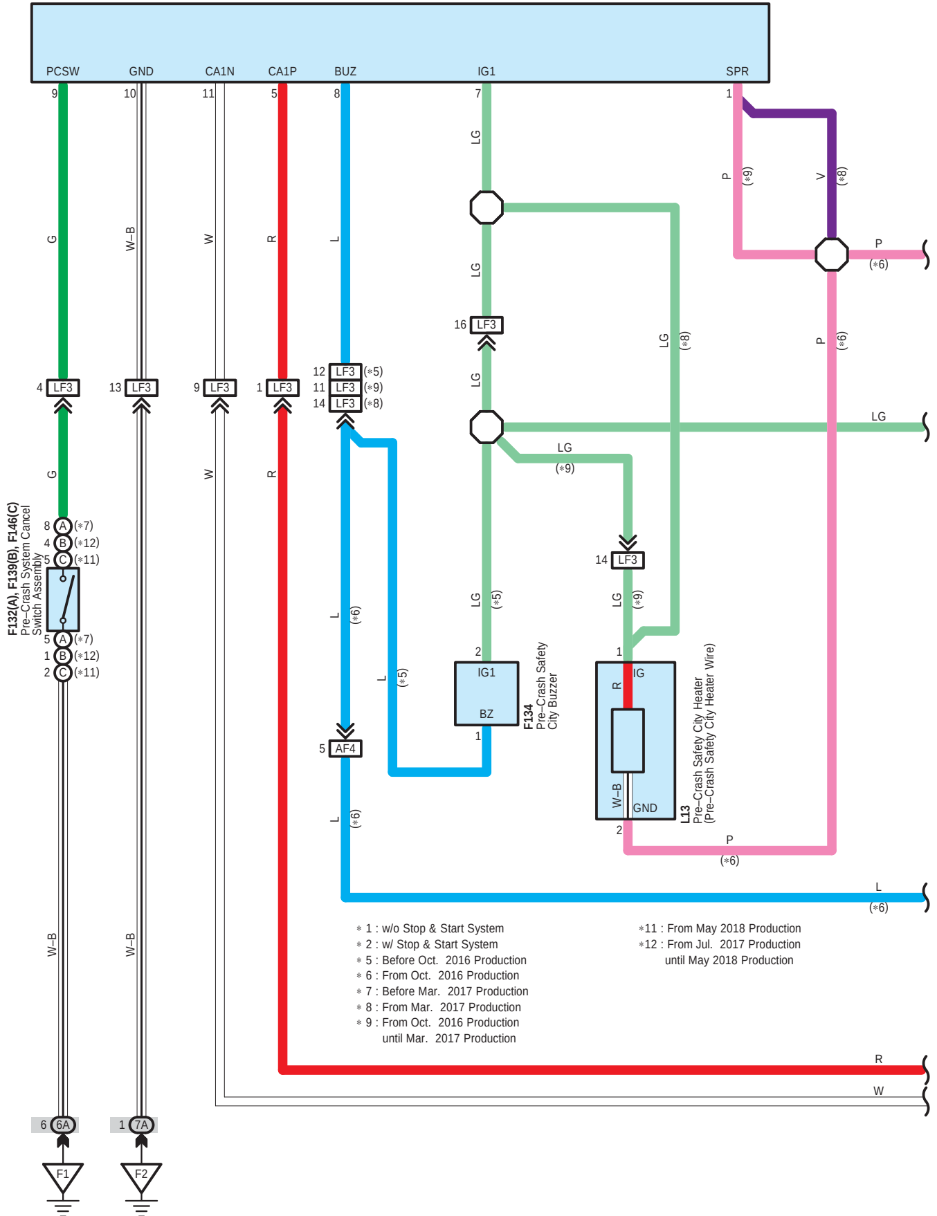
L12 Pre-Crash Safety City Sensor
