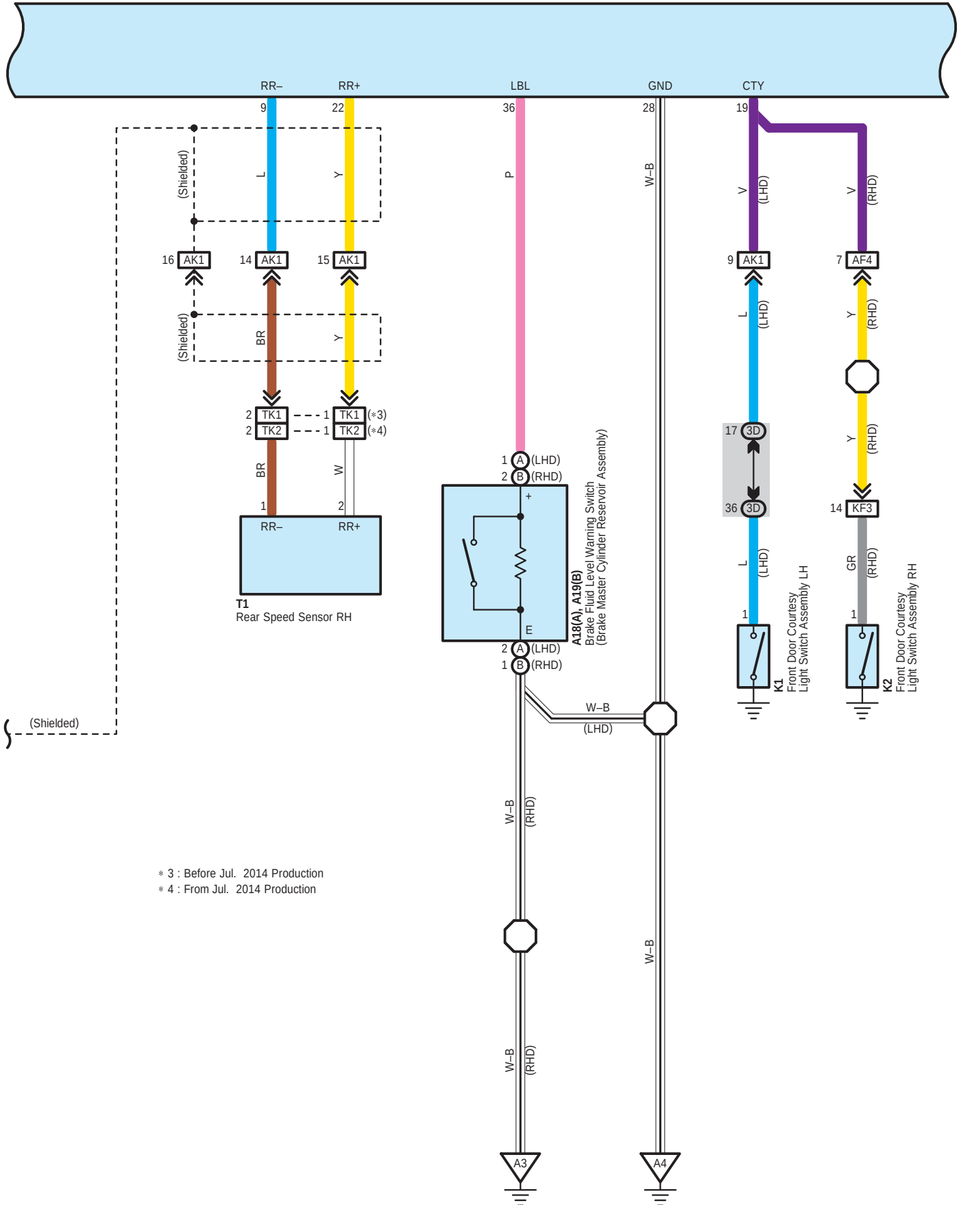
A29 Skid Control ECU with Actuator (Brake Booster with Master Cylinder Assembly)
