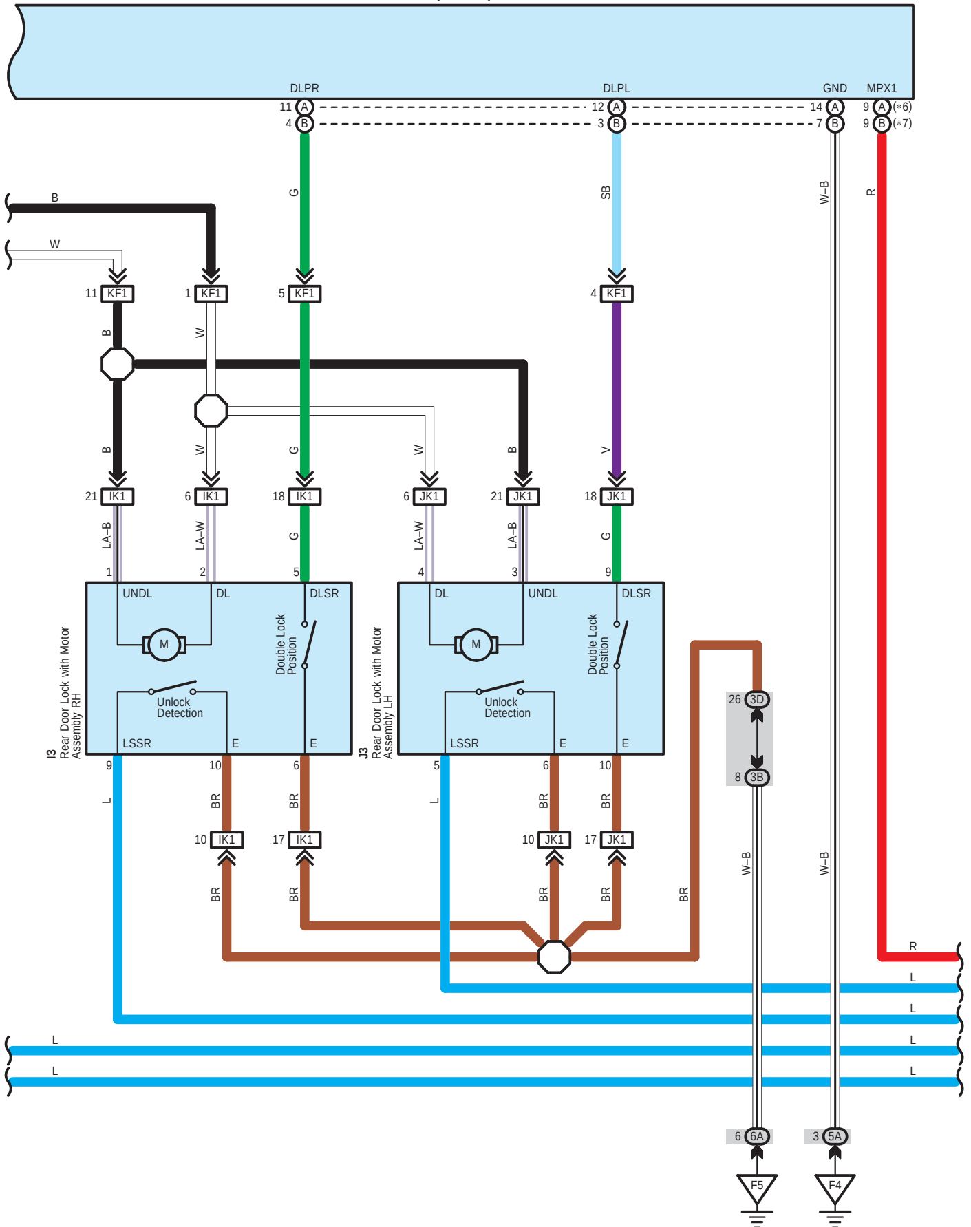
F58(A), F82(B) Double Lock Door Control Relay Assembly
