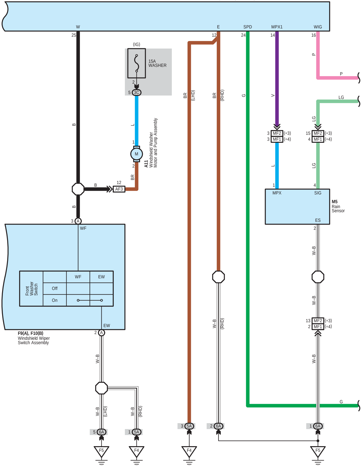
F52 Windshield Wiper Relay Assembly
