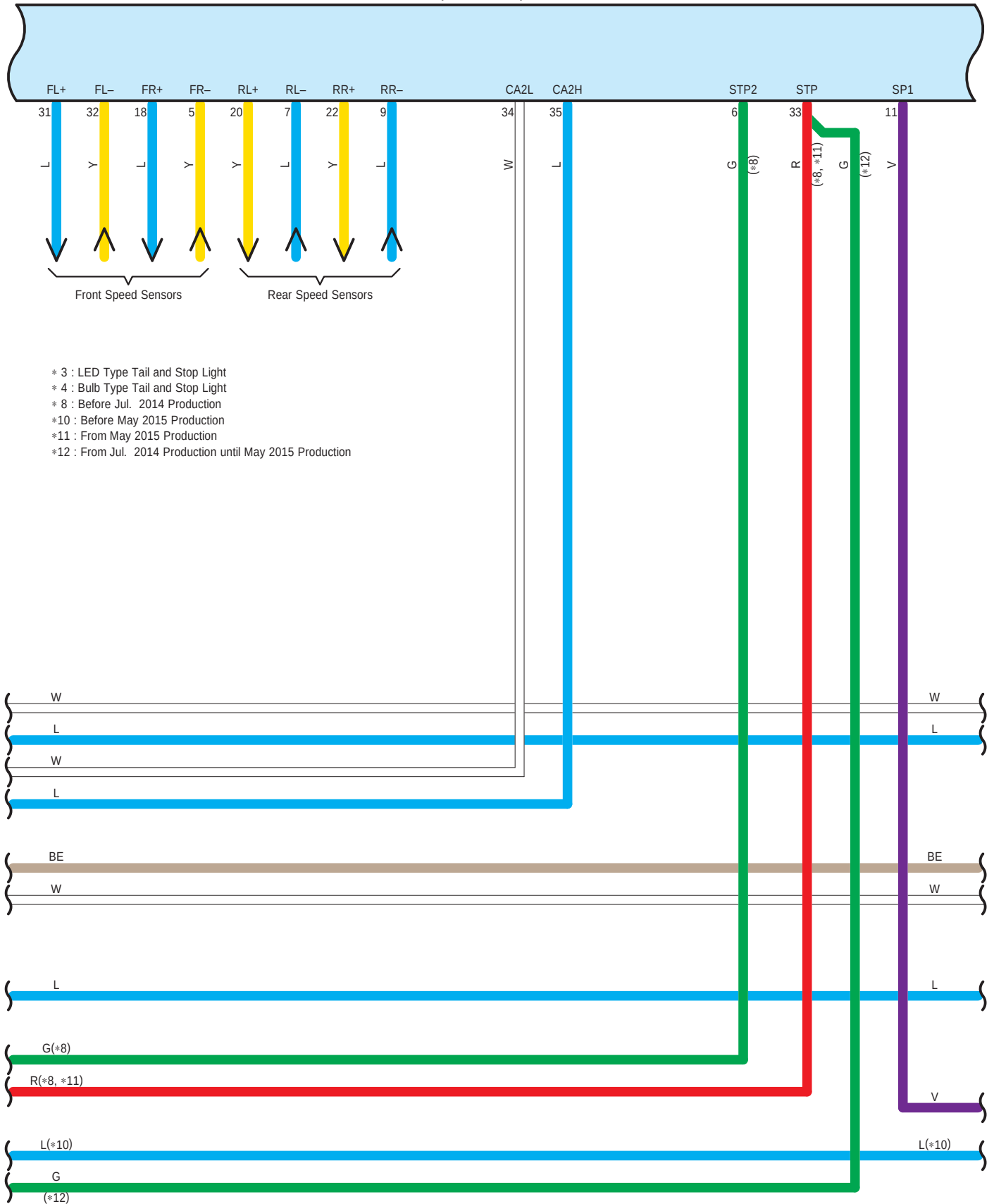
A29 Skid Control ECU with Actuator (Brake Booster with Master Cylinder Assembly)
