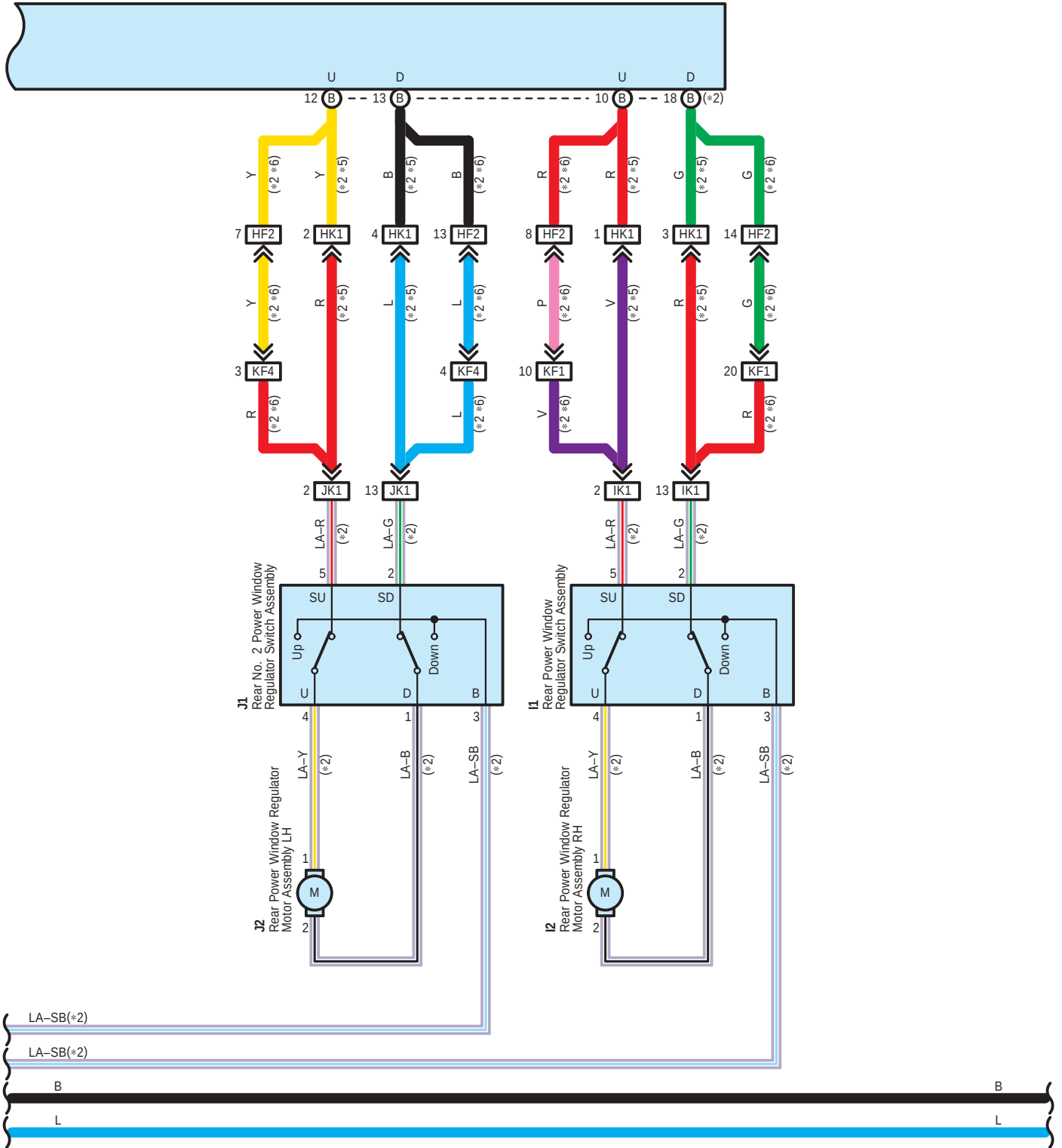
H1(A), (B) Power Window Regulator Master Switch Assembly
