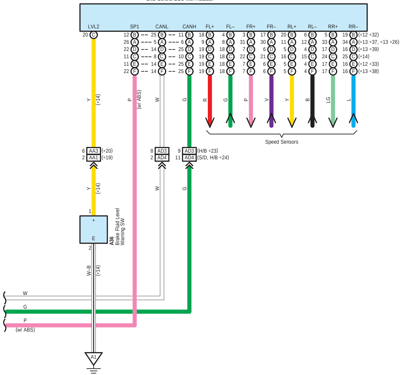
A15(A), (D), A31(B), (E), A39(C), A76(F) Skid Control ECU with Actuator
