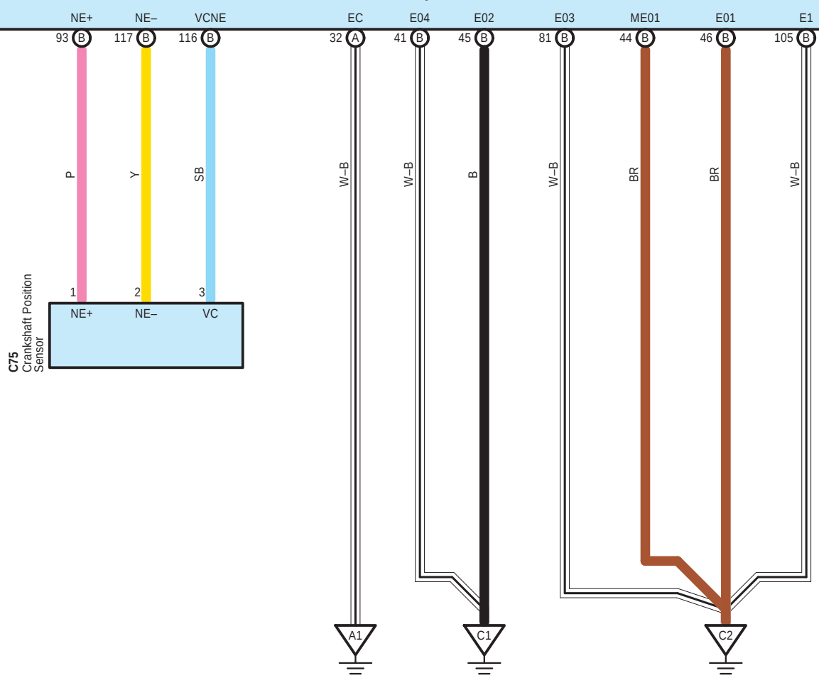
A21(A), C20(B) Engine ECU
