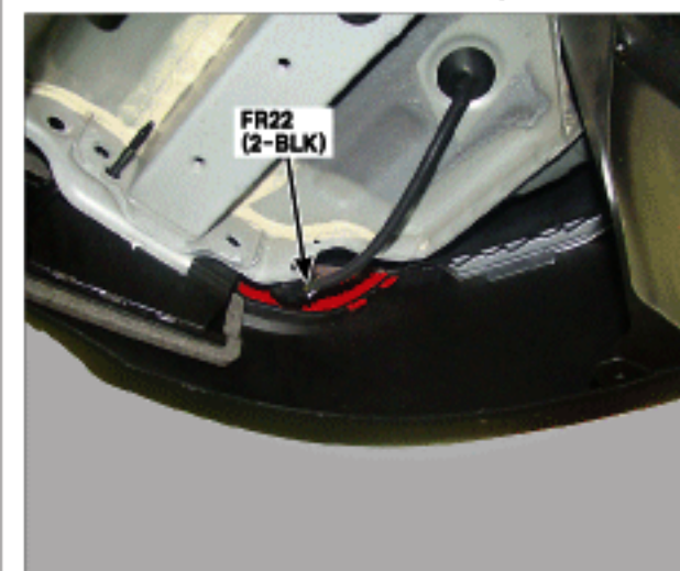
127. Left Under of Rear Bumper
