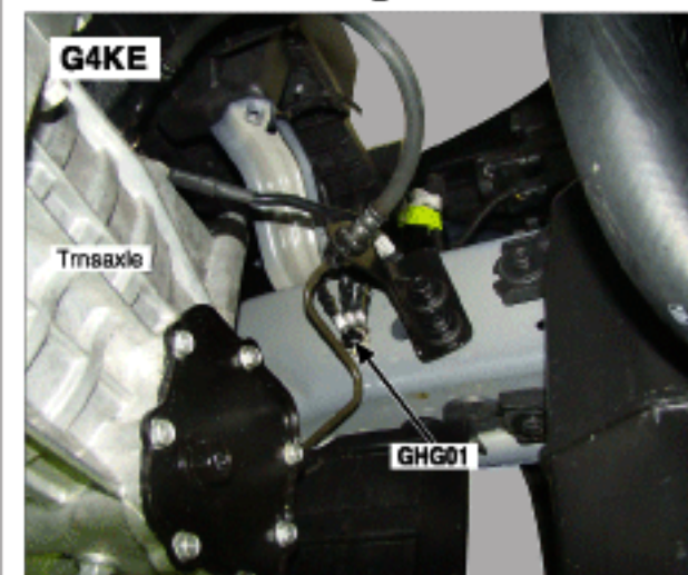
130. Left Front of Engine Room
