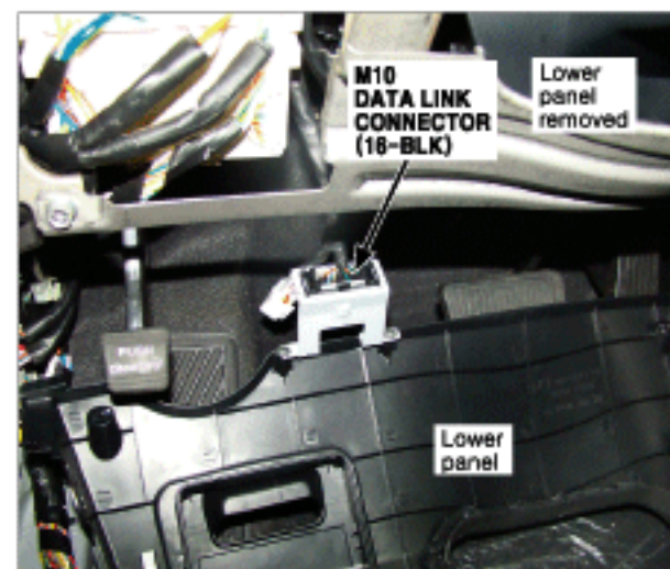
51. Dash Lower Panel
