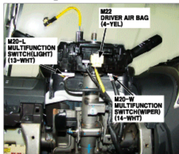
35. Steering Column
