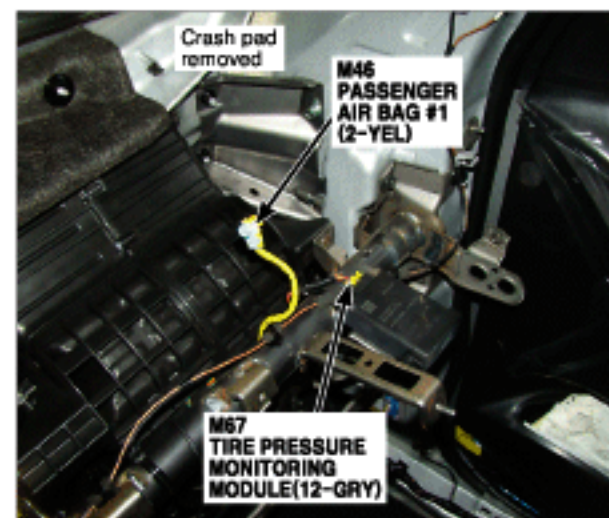
75. Right Top of Dash Panel
