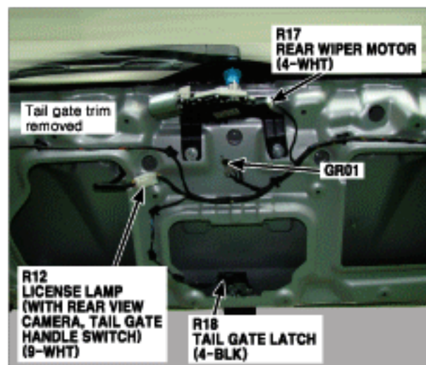
122. Tail Gate
