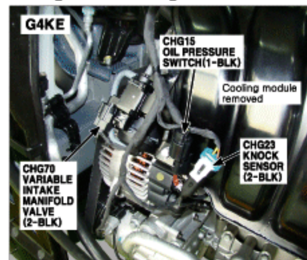
24. Right Front of Engine
