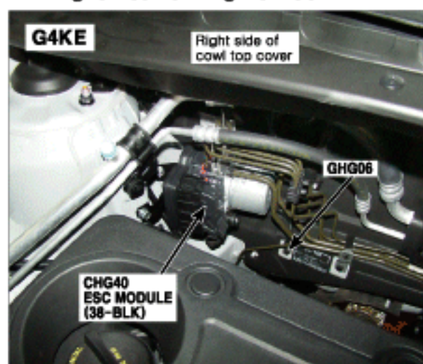
14. Right Rear of Engine Room
