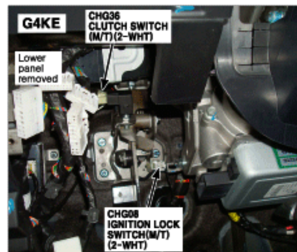
54. Left Under of Dash Panel
