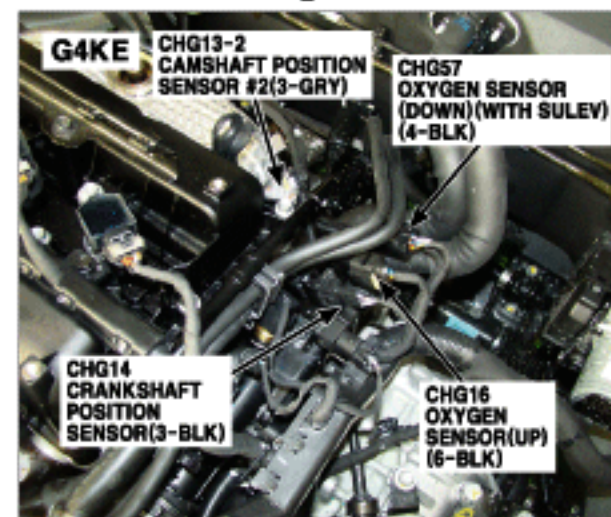
30. Left Side of Engine
