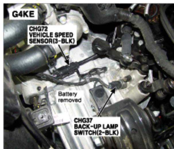
128. Top of Transaxle
