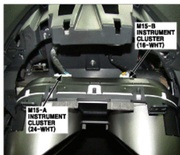
44. Instrument Cluster
