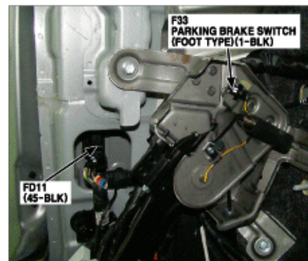
49. Under of Left A-pillar
