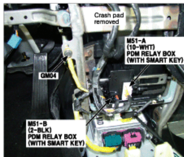
83. Center Under of Dash Panel
