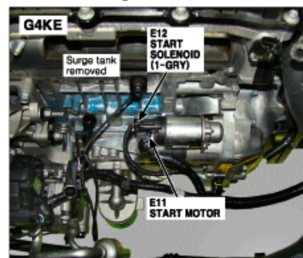
27. Front of Engine
