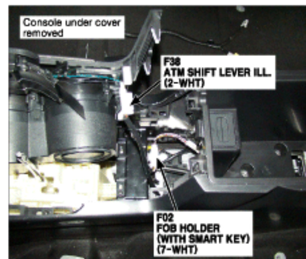
91. Center of Console
