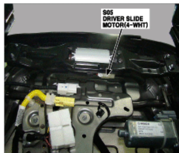
98. Under of driver seat
