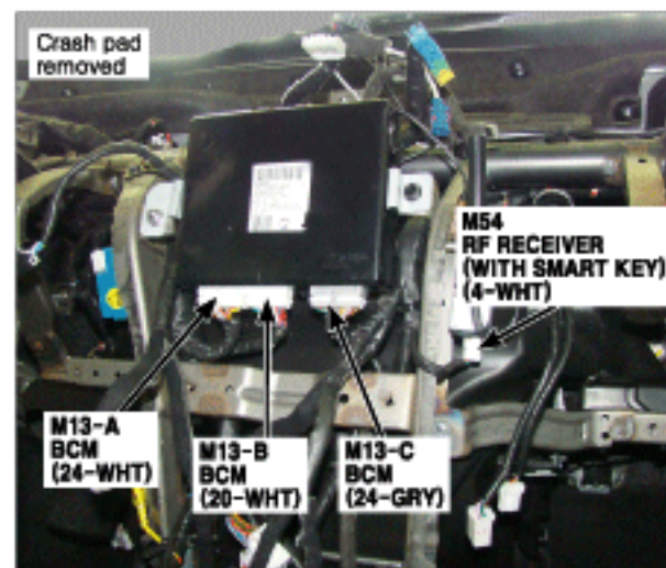
71. Center of Dash Panel
