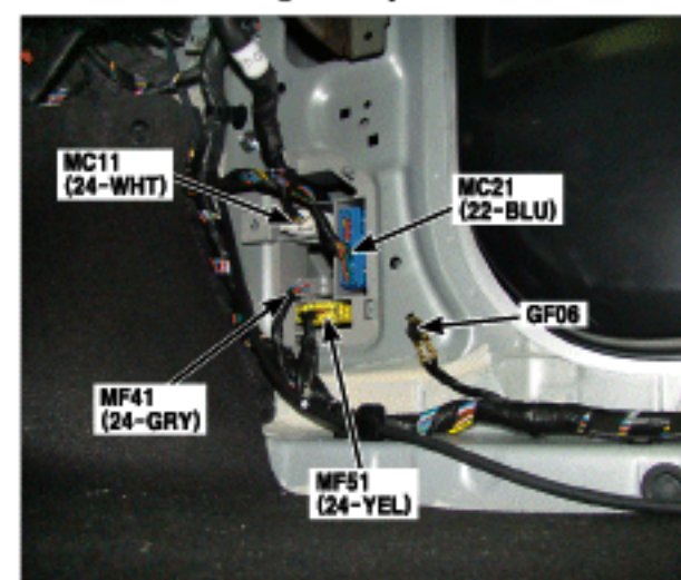
81. Under of Right A-pillar
