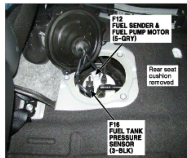
100. Left Side of Rear Seat Cushion
