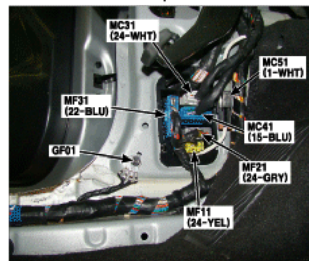
52. Under of Left A-pillar
