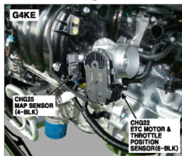
26. Left Front of Engine
