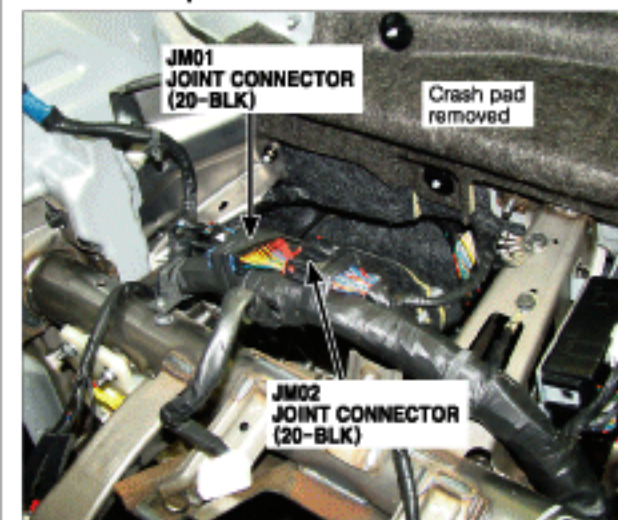
46. Left Top of Dash Panel
