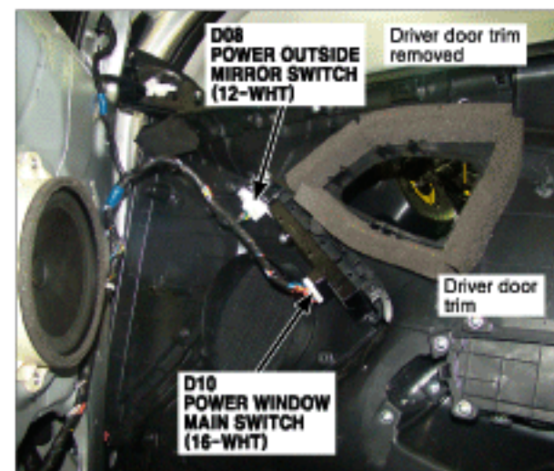
118. Driver Door Trim
