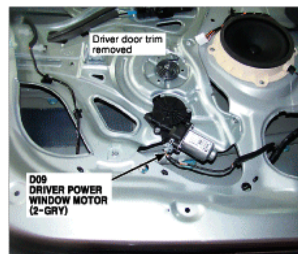
9. Driver Door
