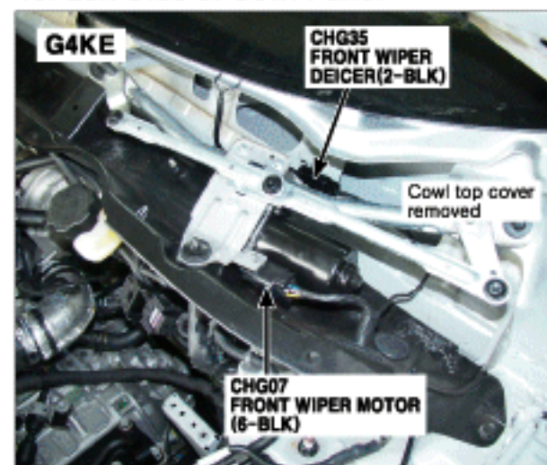
18. Left Side of Cowl Panel
