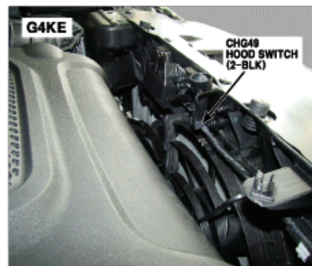
33. Front of Engine Room
