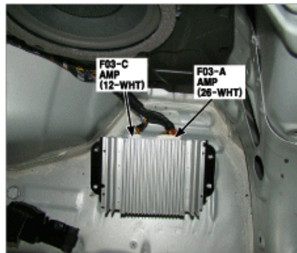
107. Right Under of Luggage Panel
