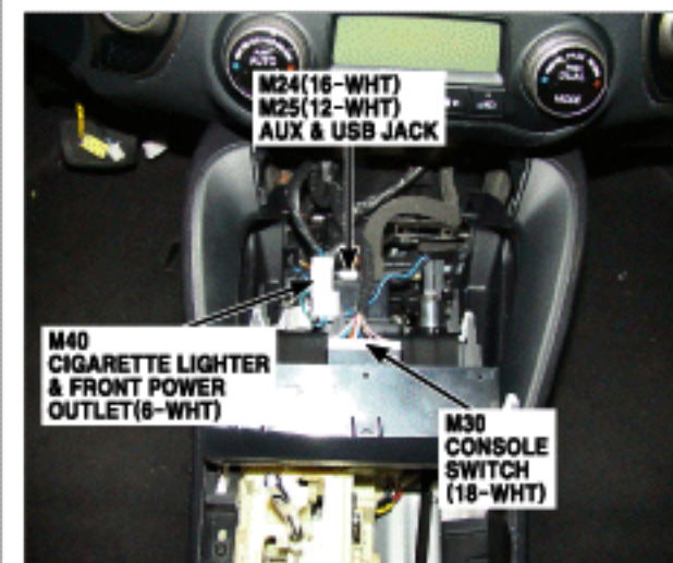
82. Front of Console
