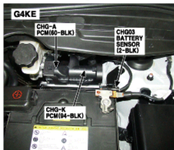
32. Left Rear of Engine Room
