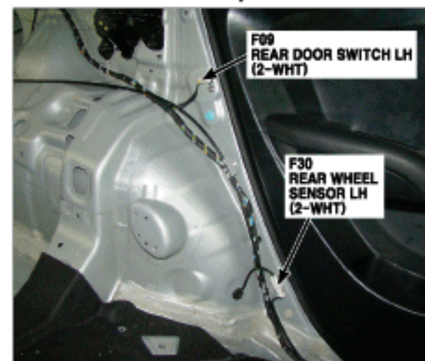
102. Under of Left C-pillar
