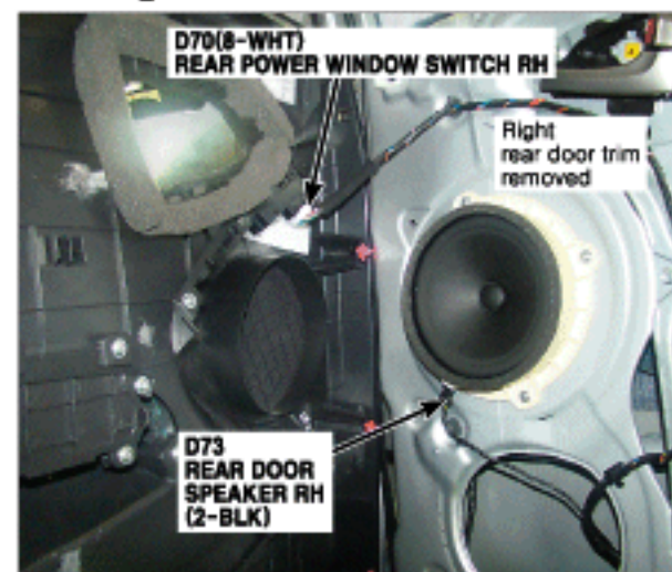
120. Right Side of Rear Door
