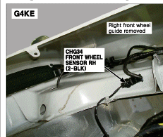
19. Right Front Wheel Housing
