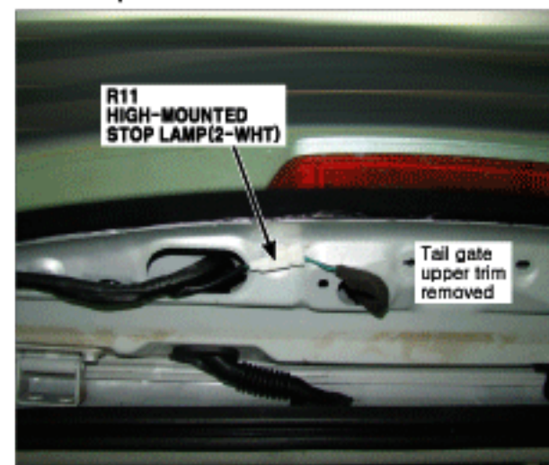
124. Top of Tail Gate
