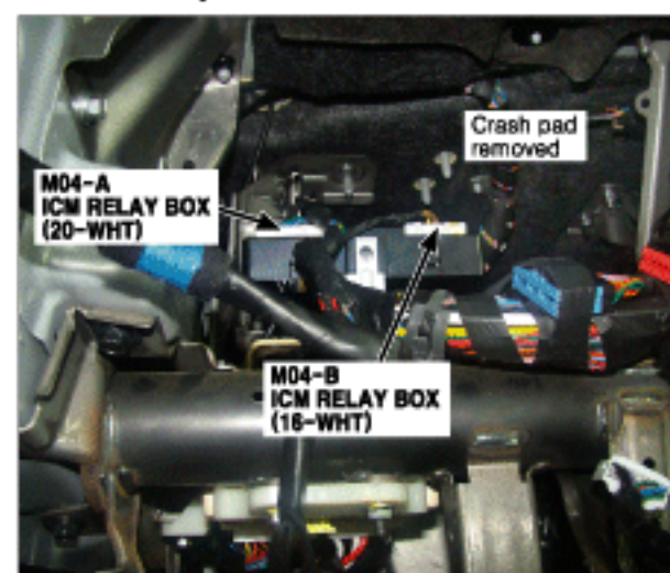
45. Left Top of Dash Panel
