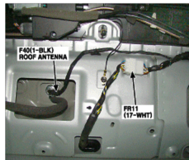
121. Rear of Roof Panel
