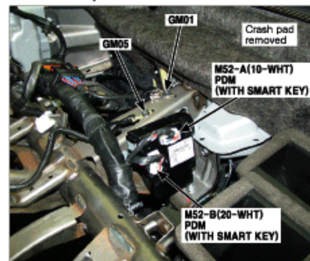
66. Left Top of Dash Panel
