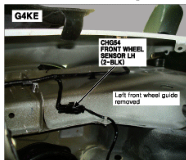
20. Left Front Wheel Housing
