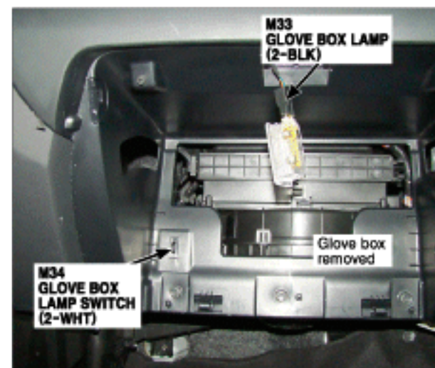
76. Inside of Glove Box
