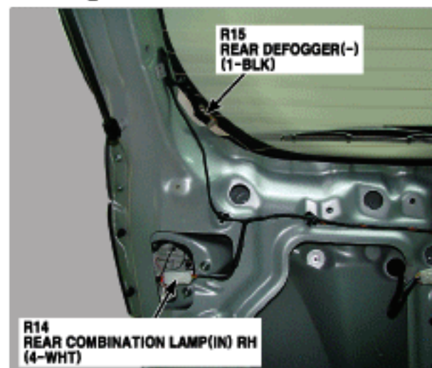
126. Right Side of Tail Gate
