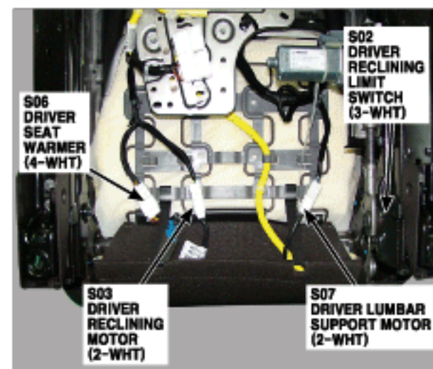
99. Under of driver seat
