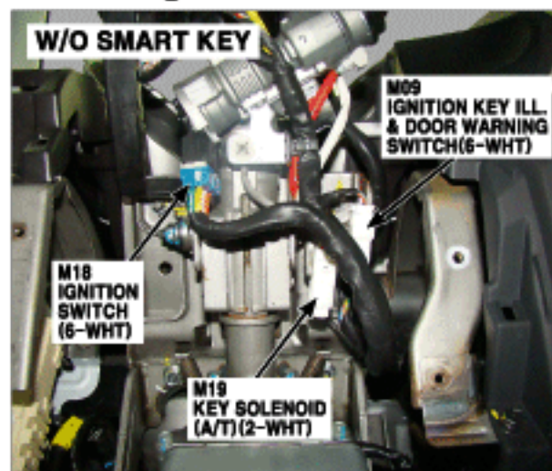
53. Steering Column
