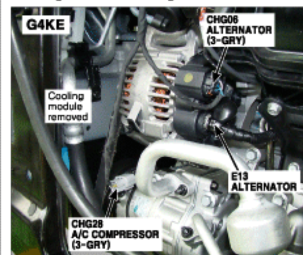
25. Right Front of Engine
