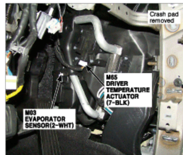
69. Center Under of Dash Panel
