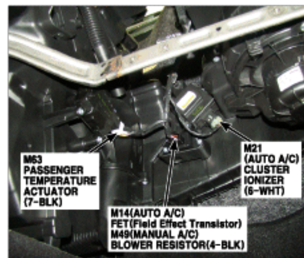
78. Center Under of Dash Panel
