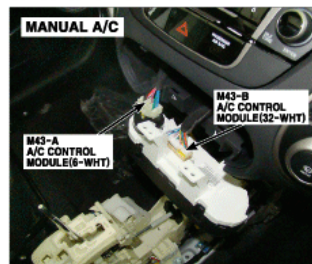
63. Center of Dash Panel
