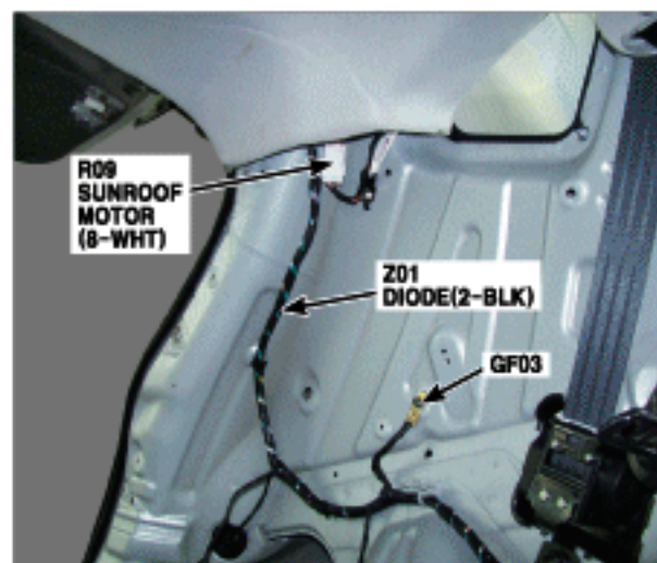
104. Left Side of Luggage Panel
