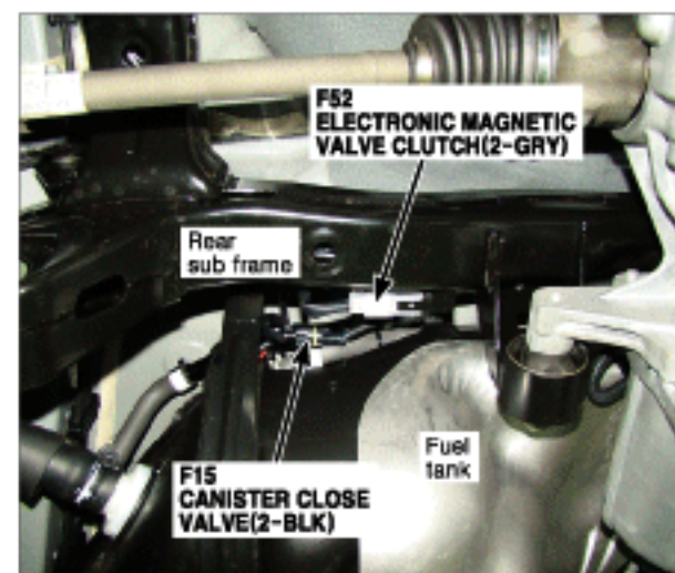
109. Rear of Fuel Tank
