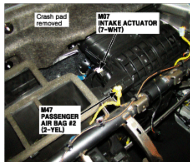
74. Center Top of Dash Panel
