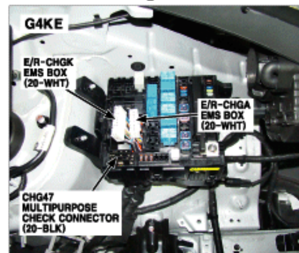
12. Left Side of Engine Room
