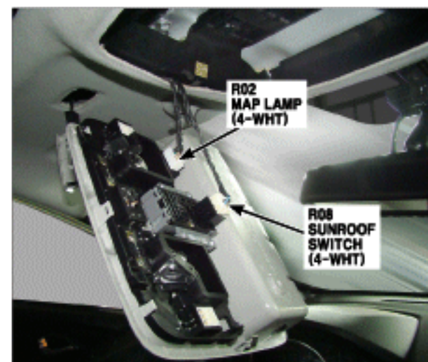
88. Front of Roof Trim
