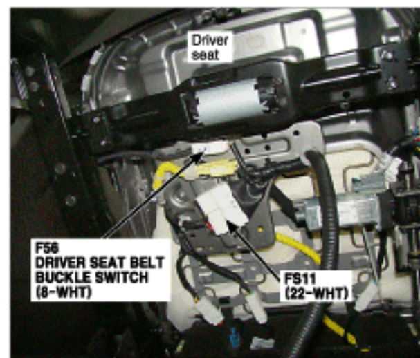
123. Under of Driver Seat
