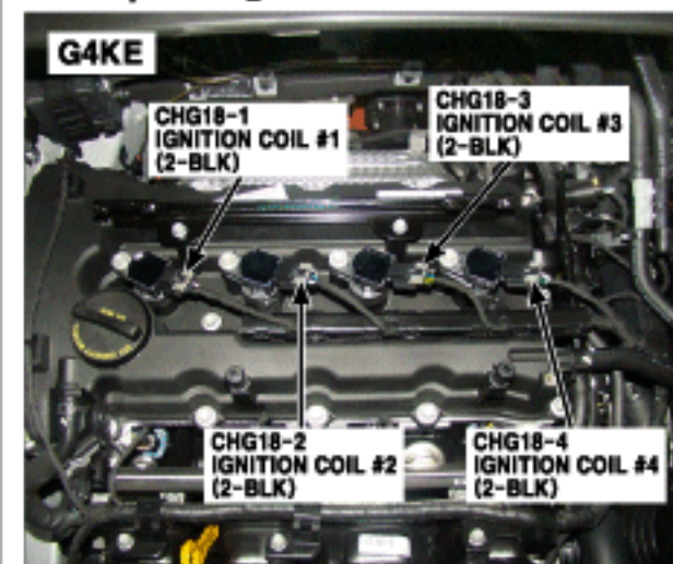
22. Top of Engine
