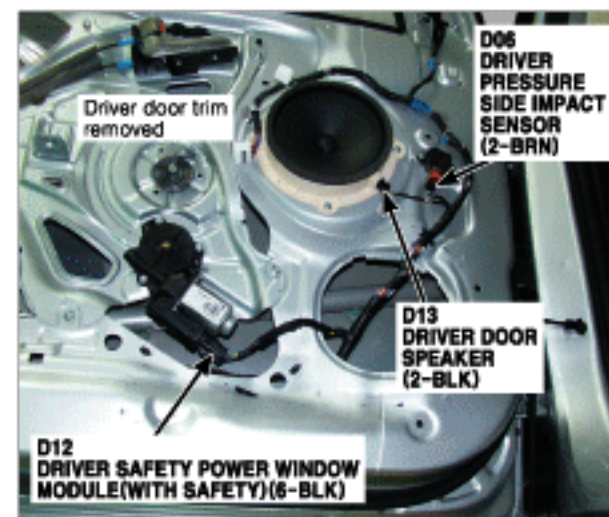
114. Driver Door
