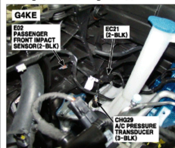
13. Right Front of Engine Room
