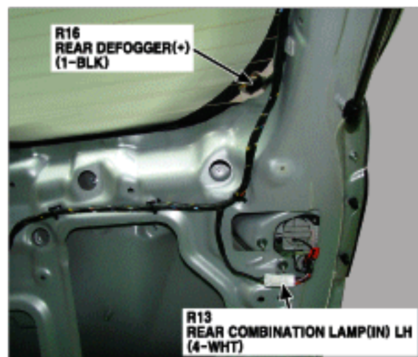
125. Left Side of Tail Gate
