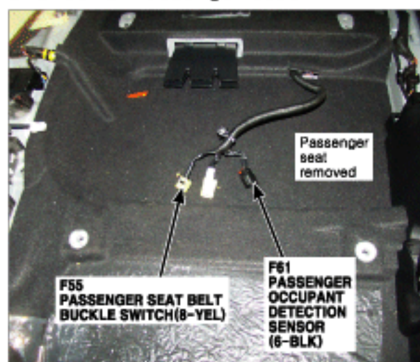
8. Under of Passenger Seat
