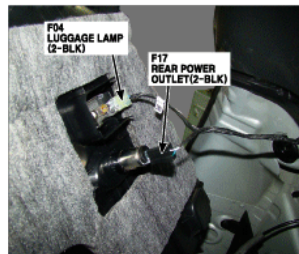
103. Left Side of Luggage Trim
