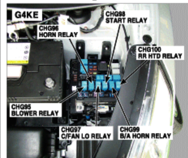
10. Left Side of Engine Room
