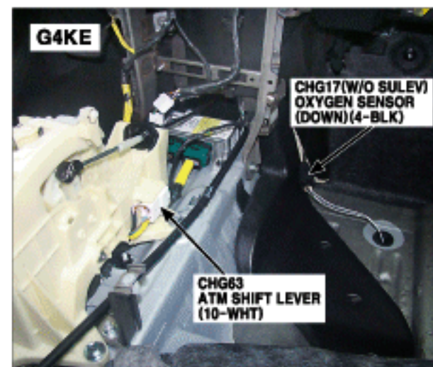
85. Center of Dash Panel
