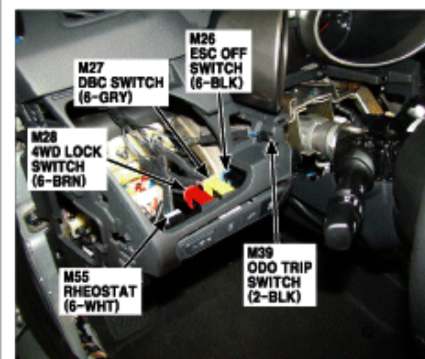
43. Left Side of Dash Panel
