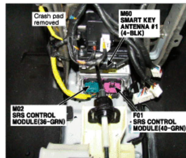
84. Center Under of Dash Panel
