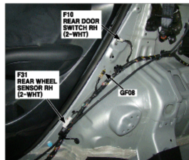
105. Under of Right C-pillar
