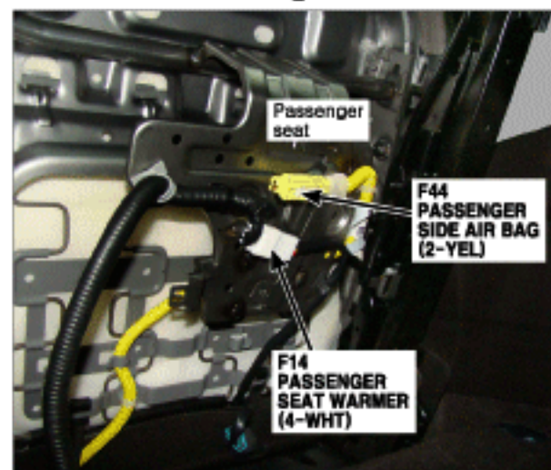
95. Under of Passenger Seat
