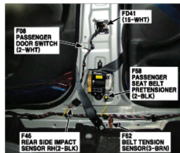
97. Right B-pillar
