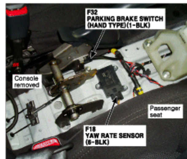
93. Center of Console
