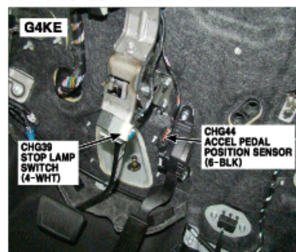
55. Left Under of Dash Panel
