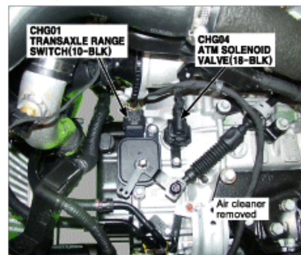
31. Top of Transaxle
