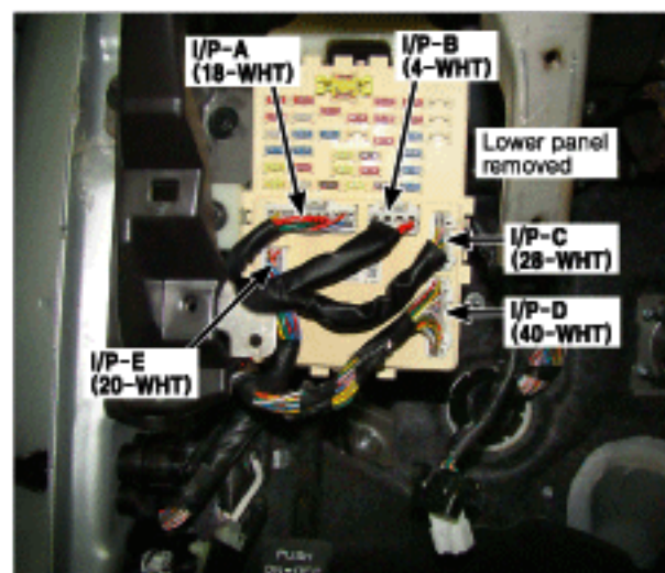
47. Left Side of Dash Panel
