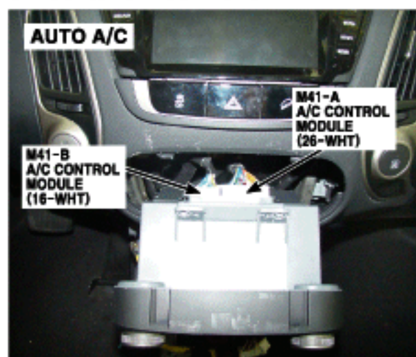
62. Center of Dash Panel
