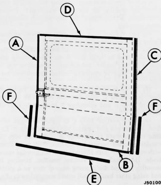
Fig. 2-33 Rubber Moulding Strips Installed
