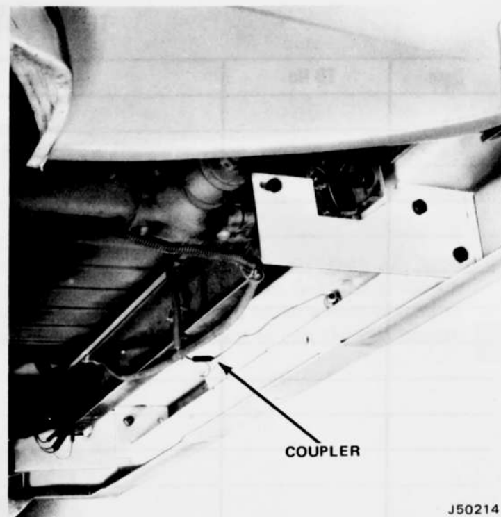
Fig. 3-13 Rear Stop Bumper—Underside View
