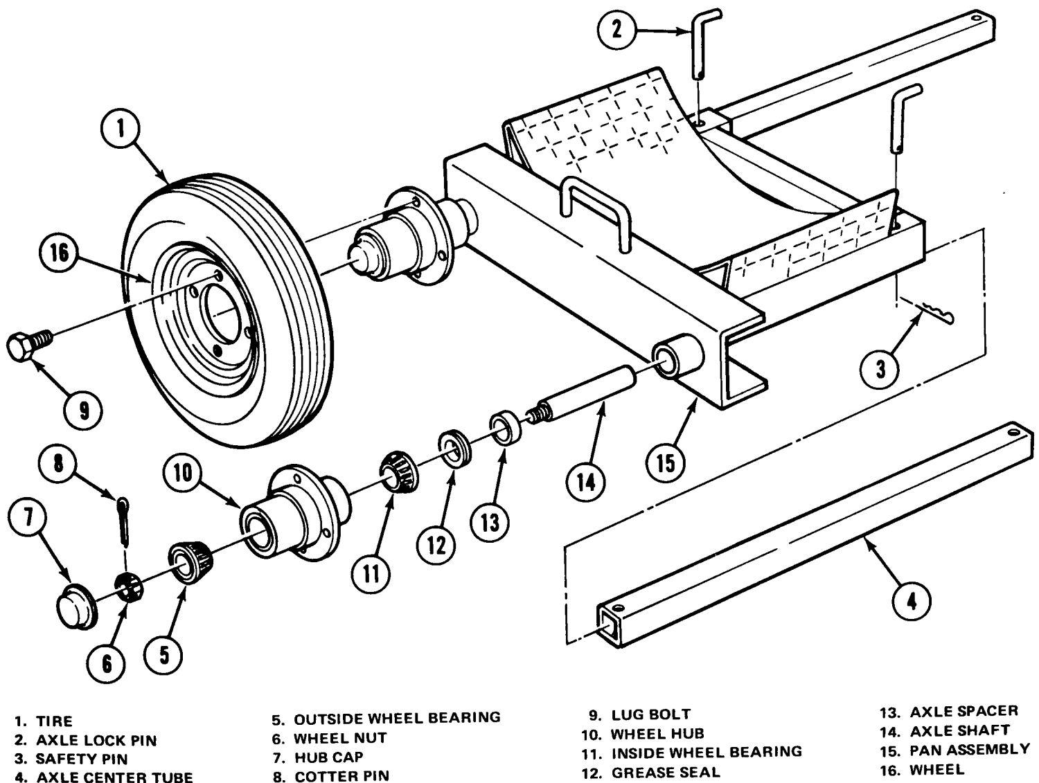
Fig. 10-12 Passenger Car Dolly—Exploded View
