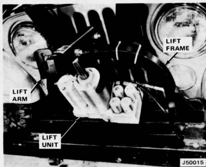
Fig. 1-19 Lift Unit—Lift Frame and Lift Arm Installation
