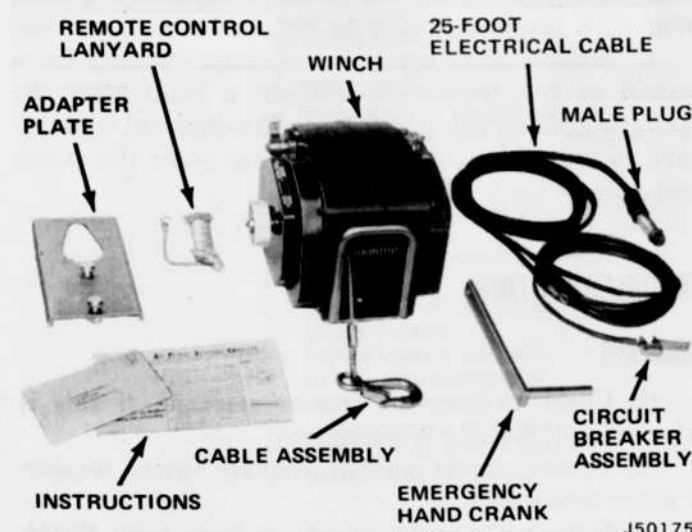
Fig. 5-35 Electric Portable Winch Kit Components
