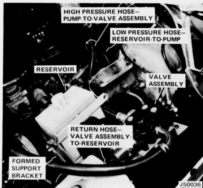
Fig. 1-54 Reservoir Installation—Cherokee-Wagoneer-Truck
