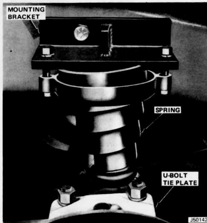
Fig. 8-4 Helper Springs Installed
