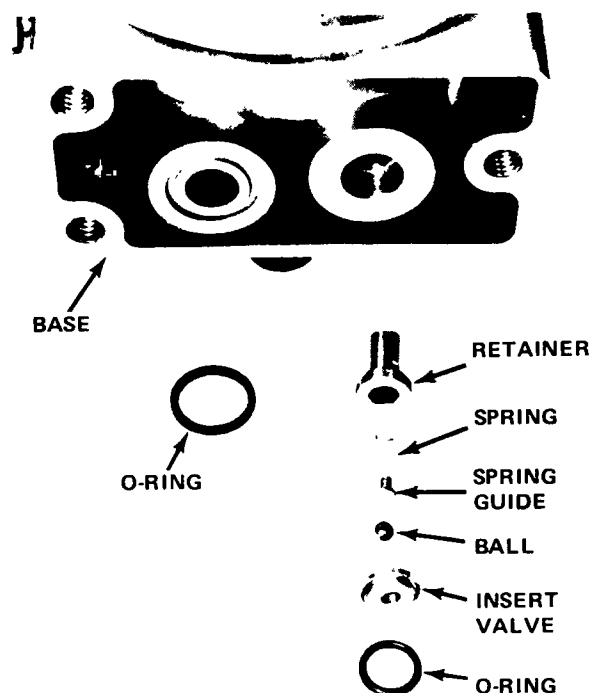
Fig. 1-28 Insert Valve—Exploded View
