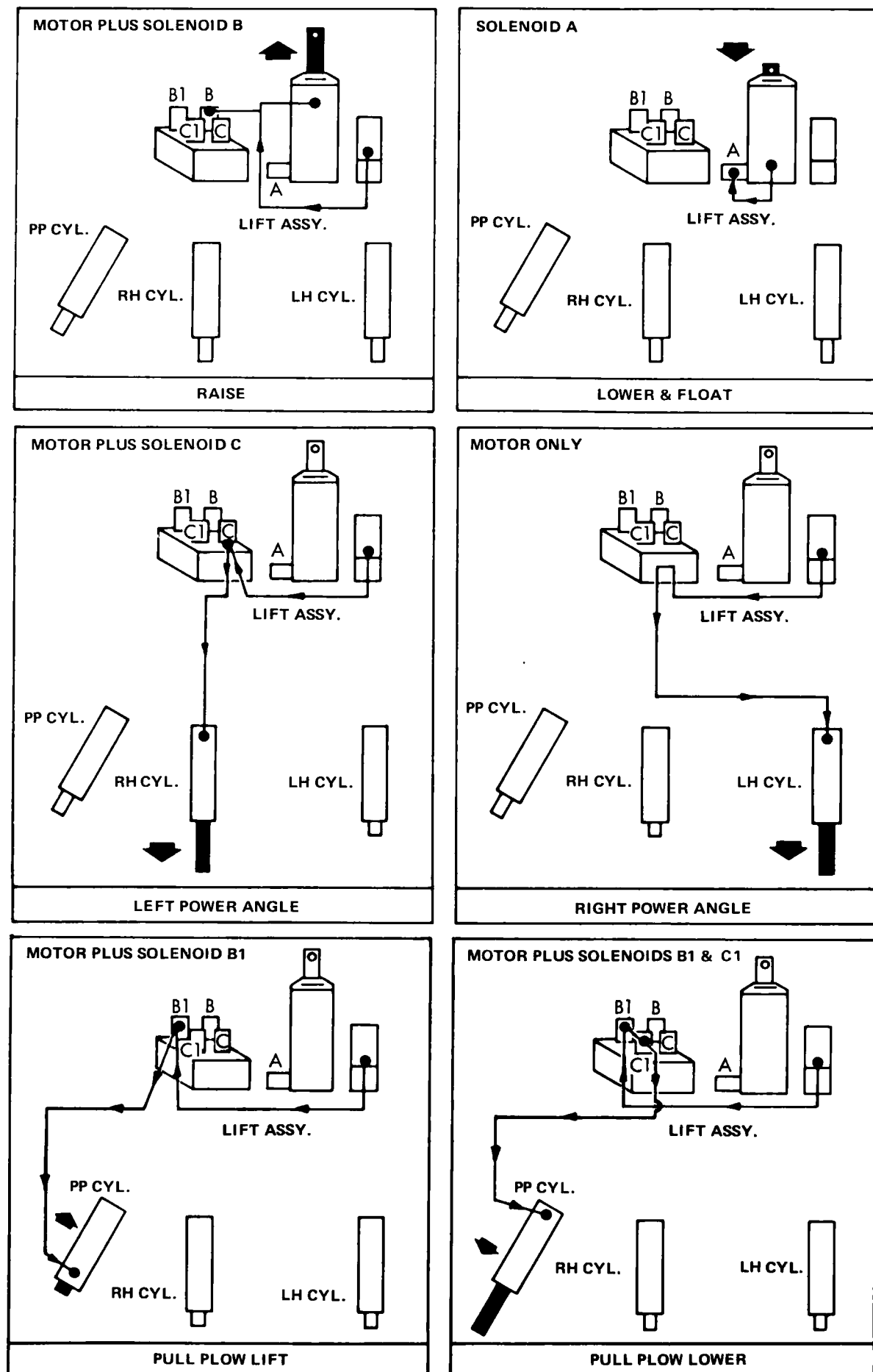
Fig. 1-26 Motor and Solenoid Valve Function Diagram
