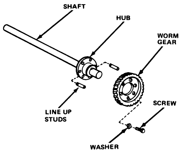
Fig. 5-31 Installing Worm Gear
