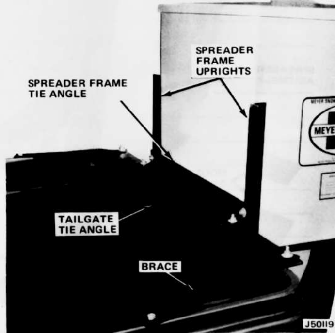
Fig. 4-3 Spreader Mounting Components
