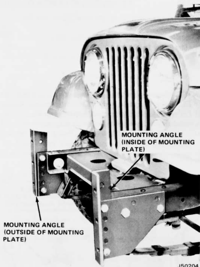
Fig. 3-3 Mounting Angles Installed
