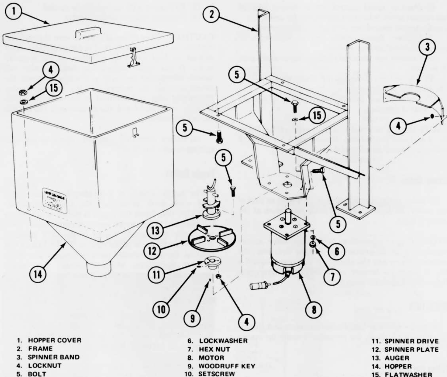
Fig. 4-10 Mini-Spreader Assembly Components and Hardware
