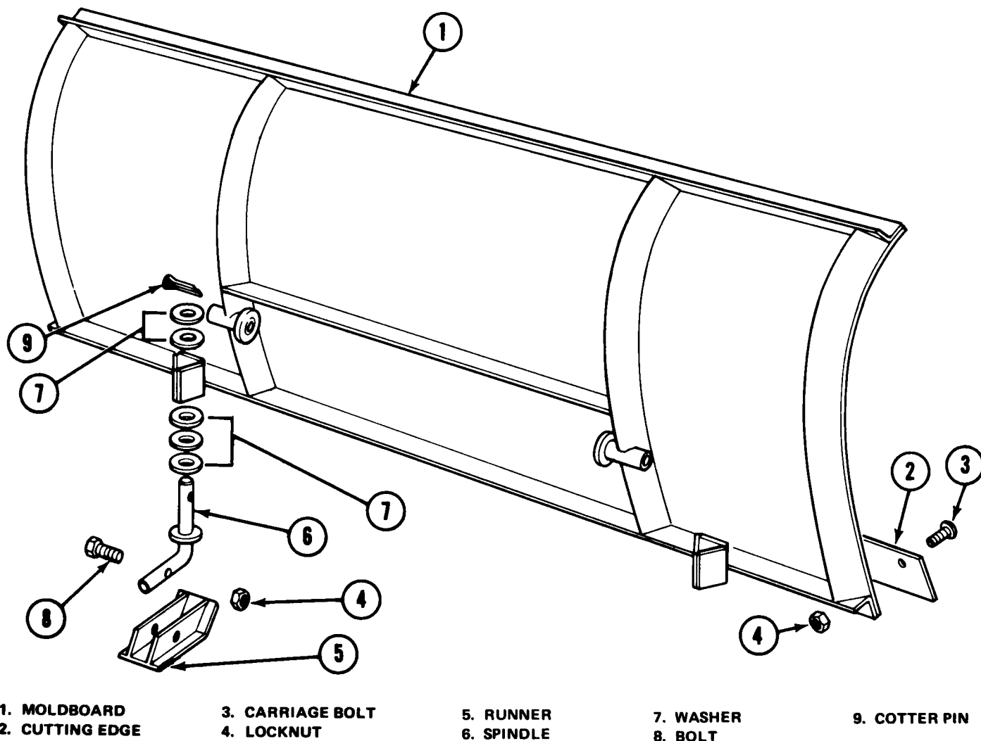
Fig. 1-8 Moldboard Assembly
