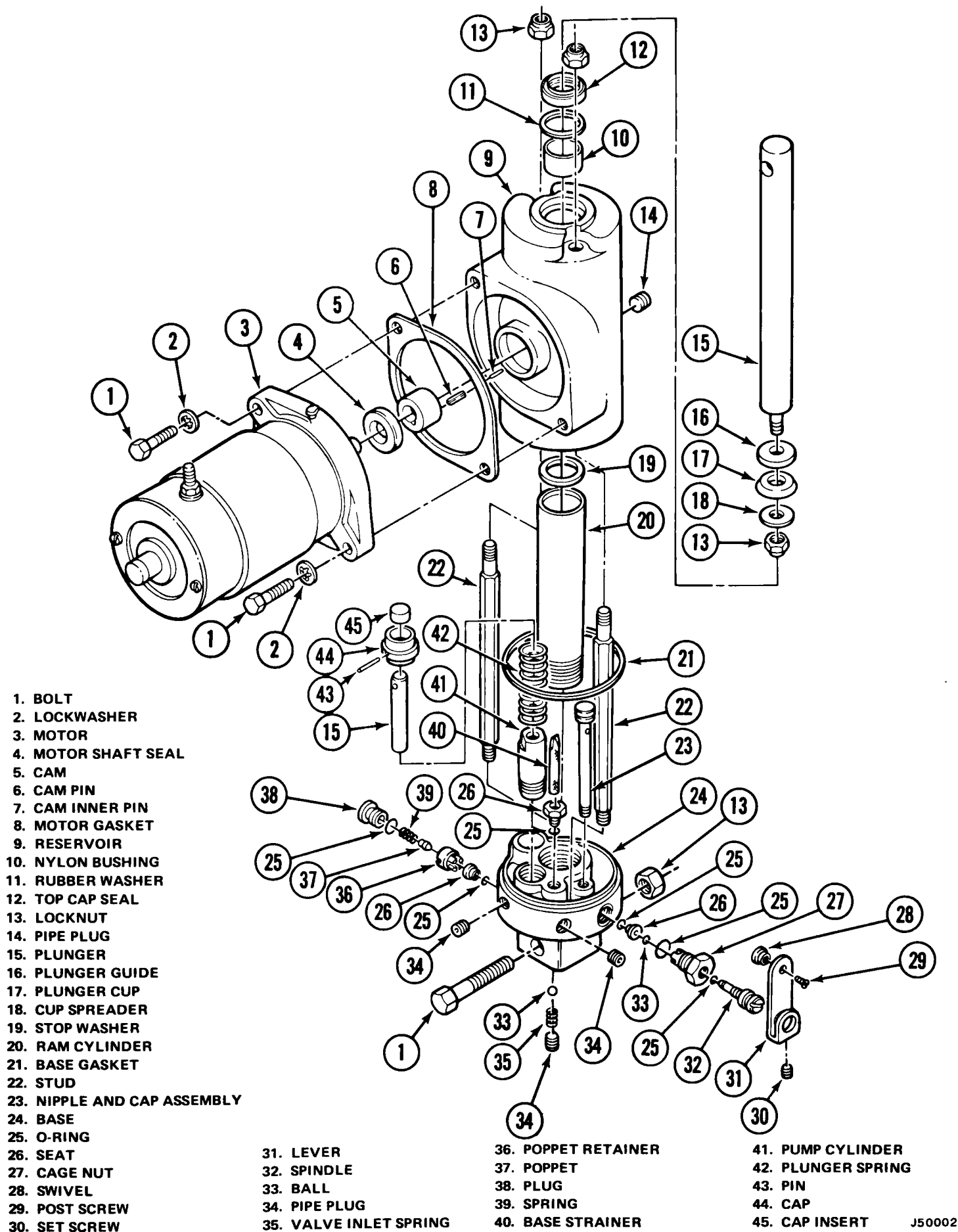
Fig. 1-35 Electrolift Model T-6—Exploded View
