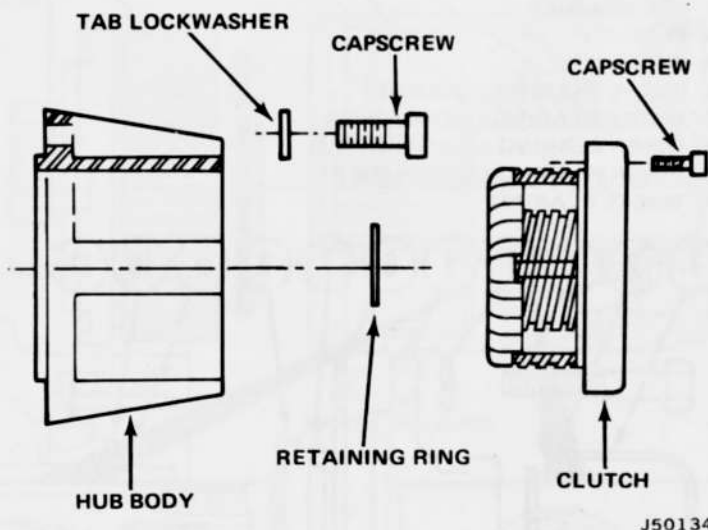
Fig. 7-2 Spring-Lock Hub—CJ Models
