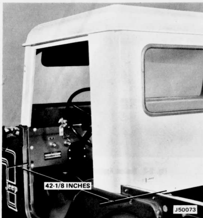
Fig. 2-5 Roof-Rear Panel Assembly Installed—Rear View
