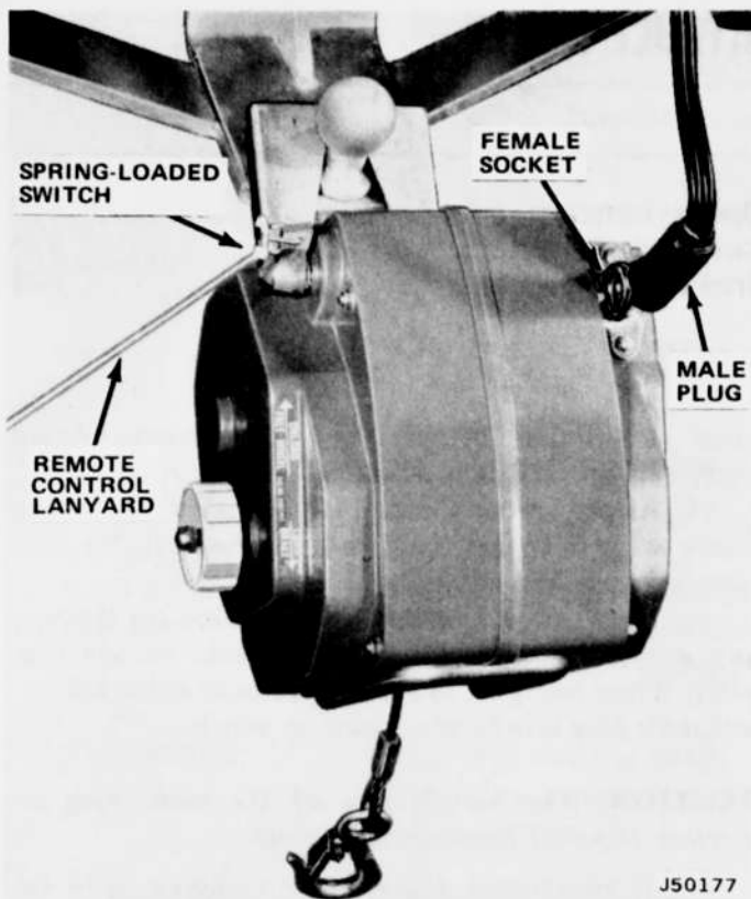
Fig. 5-37 Electric Portable Winch Installed
