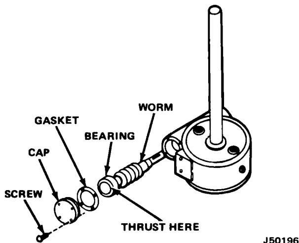
Fig. 5-32 Installing Worm
