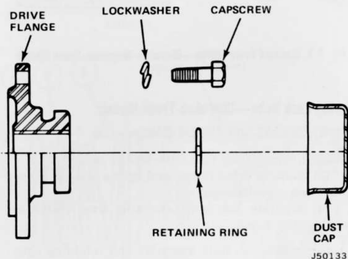
Fig. 7-1 Standard Drive Flange—CJ Models
