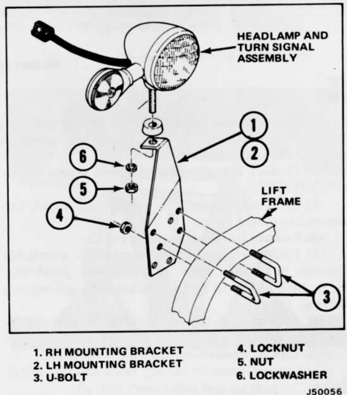
Fig. 1-16 Headlamp and Turn Signal Installation
