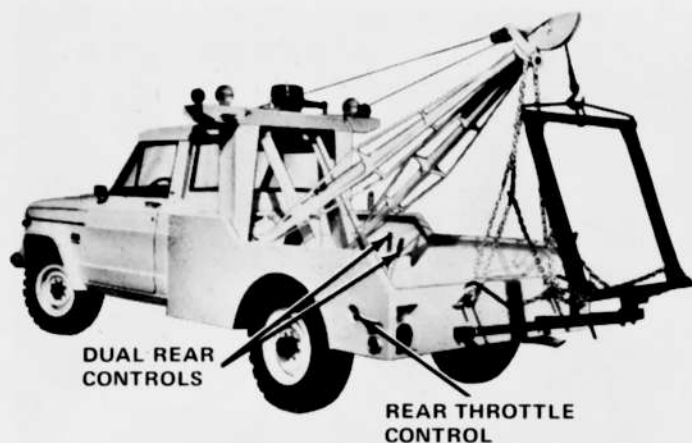
Fig. 10-8 Wrecker Kit Installed
