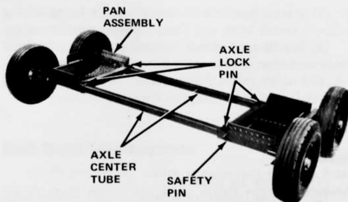
Fig. 10-11 Passenger Car Dolly—Assembled View
