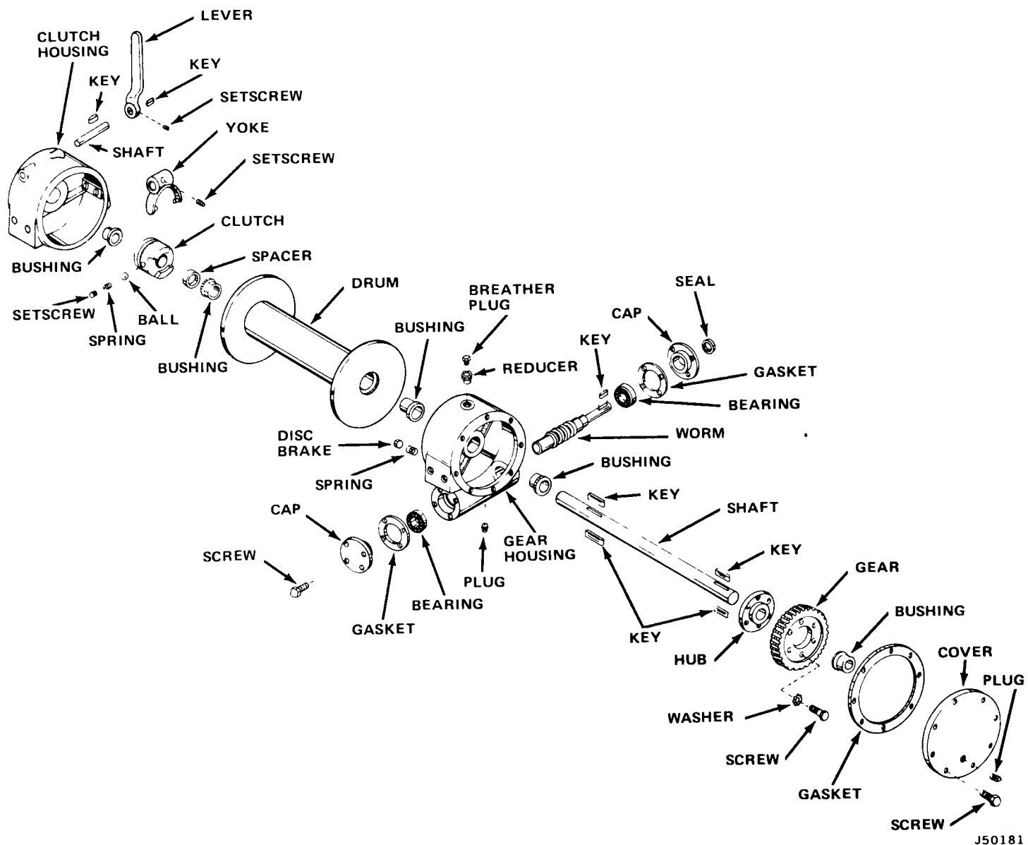
Fig. 5-17 Mechanical Winch—Exploded View
