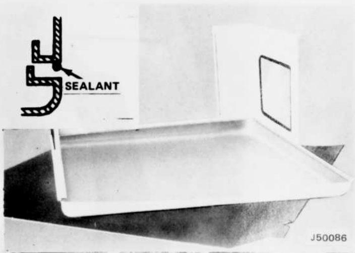
Fig. 2-18 Roof and Quarter Panels Assembled
