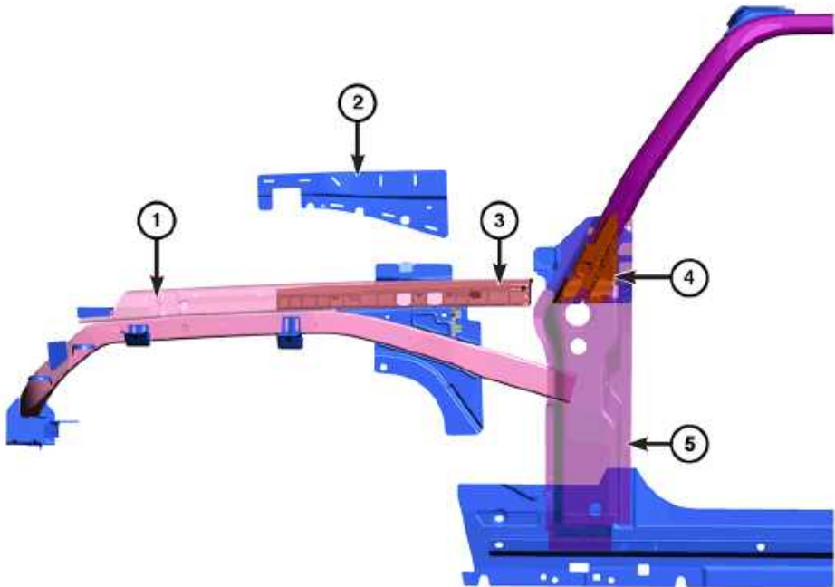
Fig. 5: A-Pillar And Upper Load Path Beam Composite Reinforcements Component Location Courtesy of CHRYSLER GROUP, LLC
