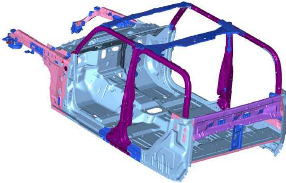
Fig. 5: Body In White (Top view rear) Structure Identification Materials Courtesy of CHRYSLER GROUP, LLC
