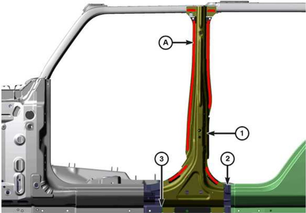
Fig. 34: B-Pillar Reinforcement and Inner B-Pillar Courtesy of CHRYSLER GROUP, LLC
