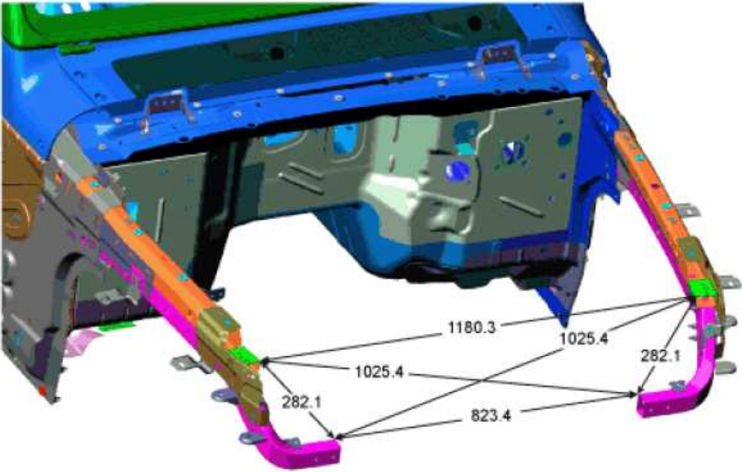
Fig. 8: Under Hood Dimensions And Measurement Points (1 of 2) Courtesy of CHRYSLER GROUP, LLC
