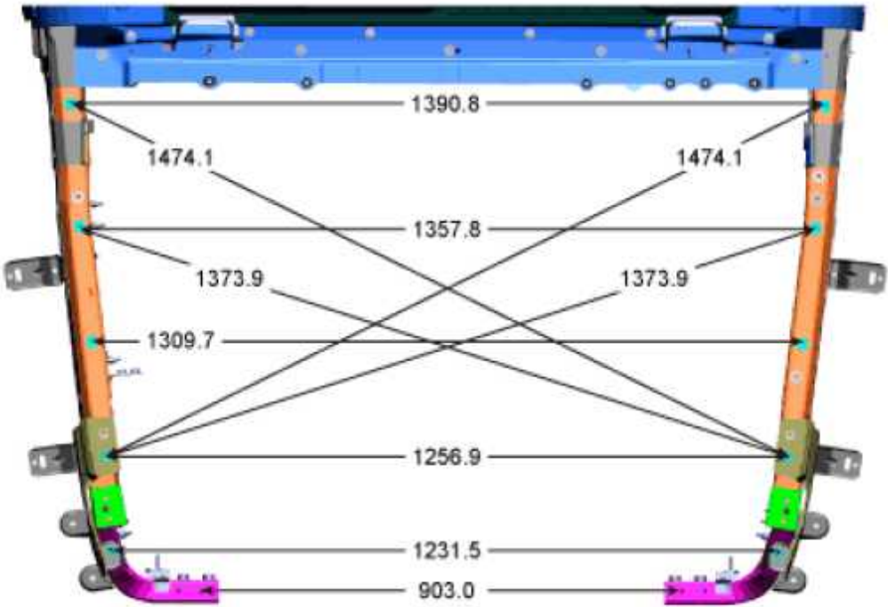
Fig. 7: Frame Dimensions And Measurement Points Courtesy of CHRYSLER GROUP, LLC
