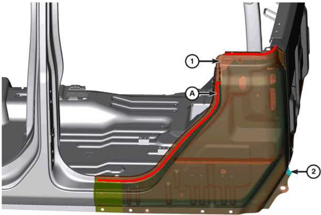
Fig. 46: Rear Body Side Aperture Courtesy of CHRYSLER GROUP, LLC
