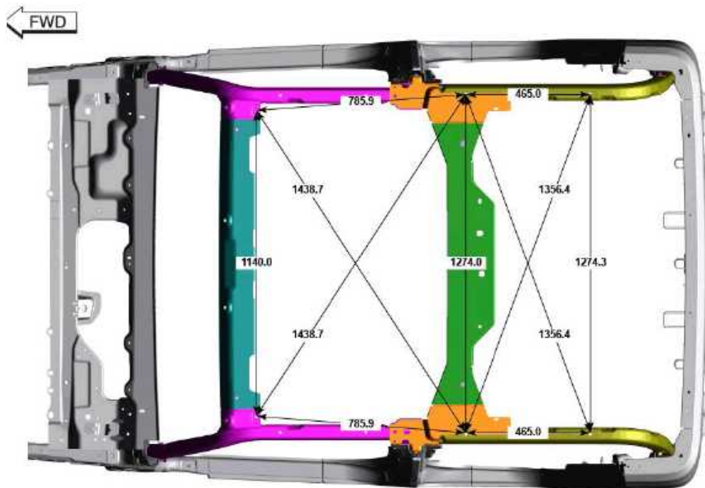
Fig. 4: Upperbody/Sport Bar Dimensions And Measurement Points Courtesy of CHRYSLER GROUP, LLC
