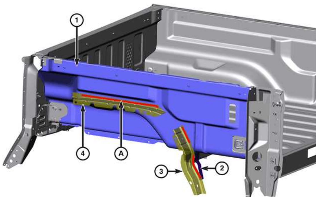
Fig. 51: Box Side Inner Panel
