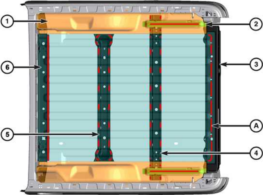
Fig. 52: Box Floor Panel Courtesy of CHRYSLER GROUP, LLC
