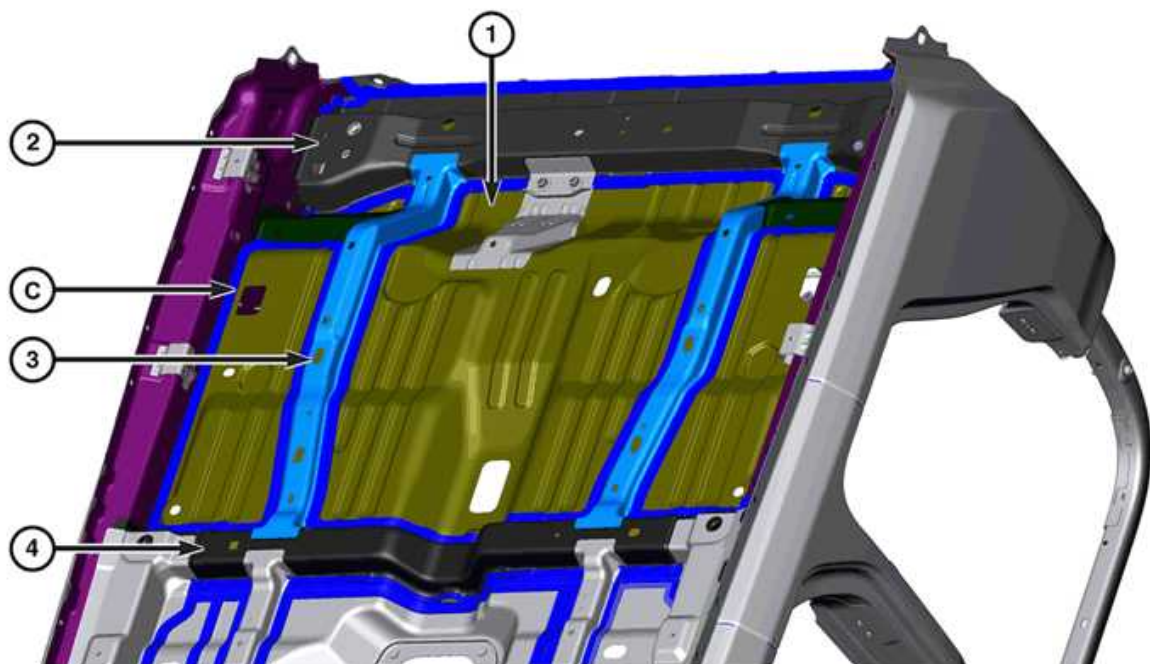
Fig. 42: Rear Floor Exterior (1 of 2)
