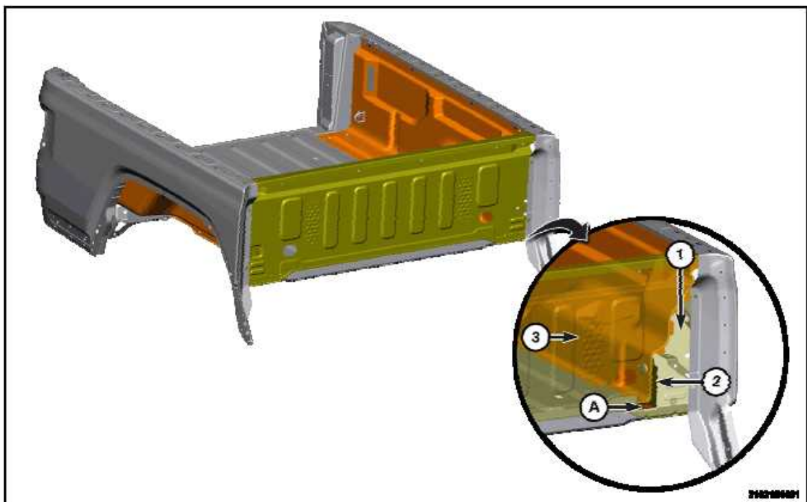
Fig. 54: Box Front Panel Courtesy of CHRYSLER GROUP, LLC
