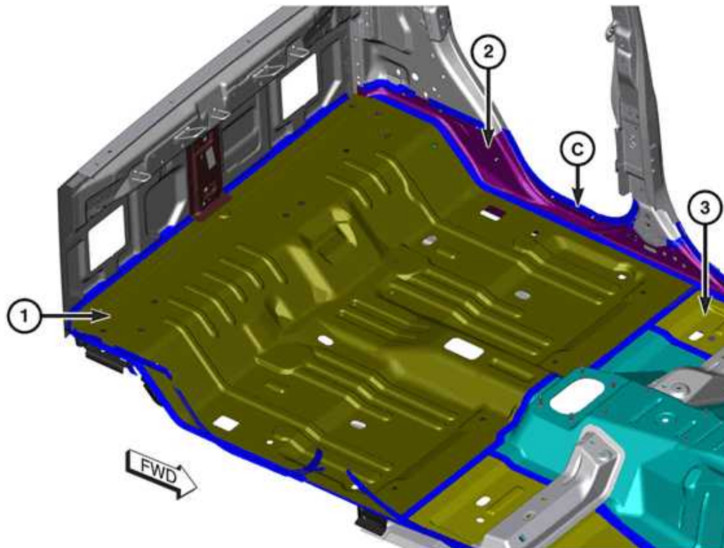
Fig. 40: Rear Floor Interior (2 of 2) Courtesy of CHRYSLER GROUP, LLC
