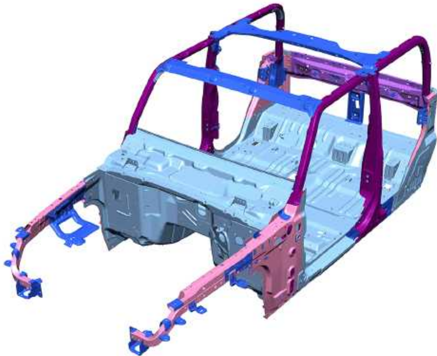
Fig. 3: Body Side Apertures, B-pillar Panel and Cab Back Panel Structure Identification Materials Courtesy of CHRYSLER GROUP, LLC
