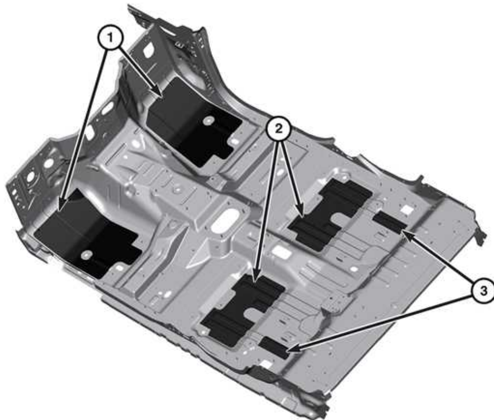
Fig. 10: Floor Pan Interior
