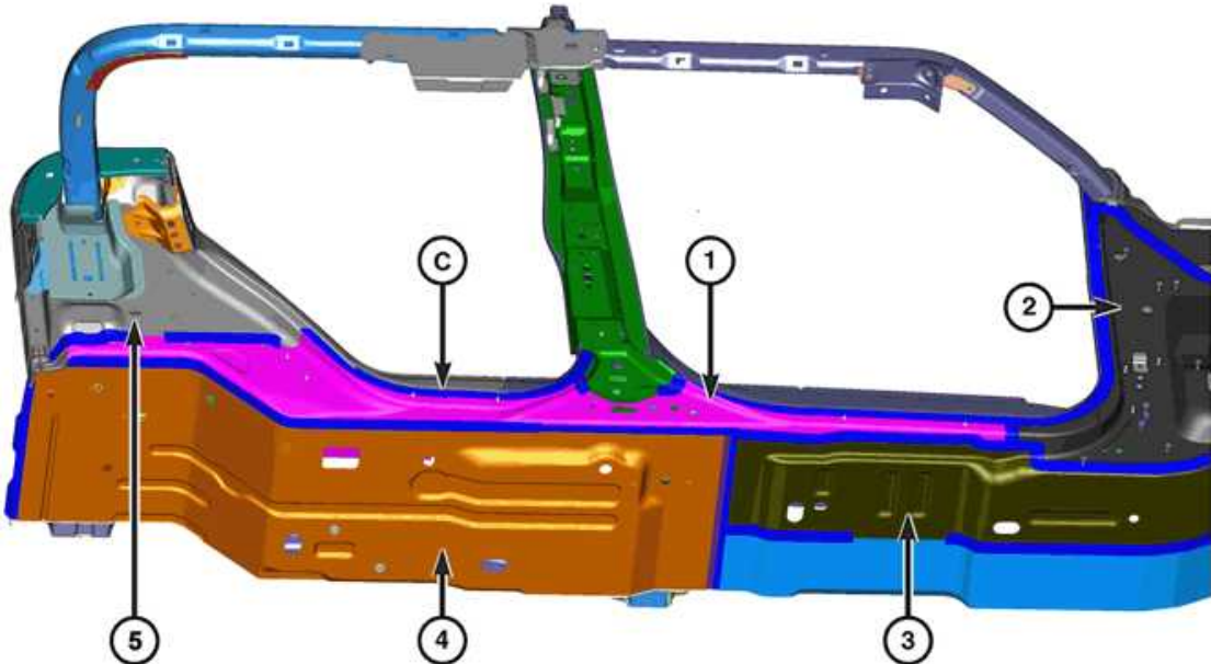
Fig. 31: Inner Sill and Floor Panels Courtesy of CHRYSLER GROUP, LLC
