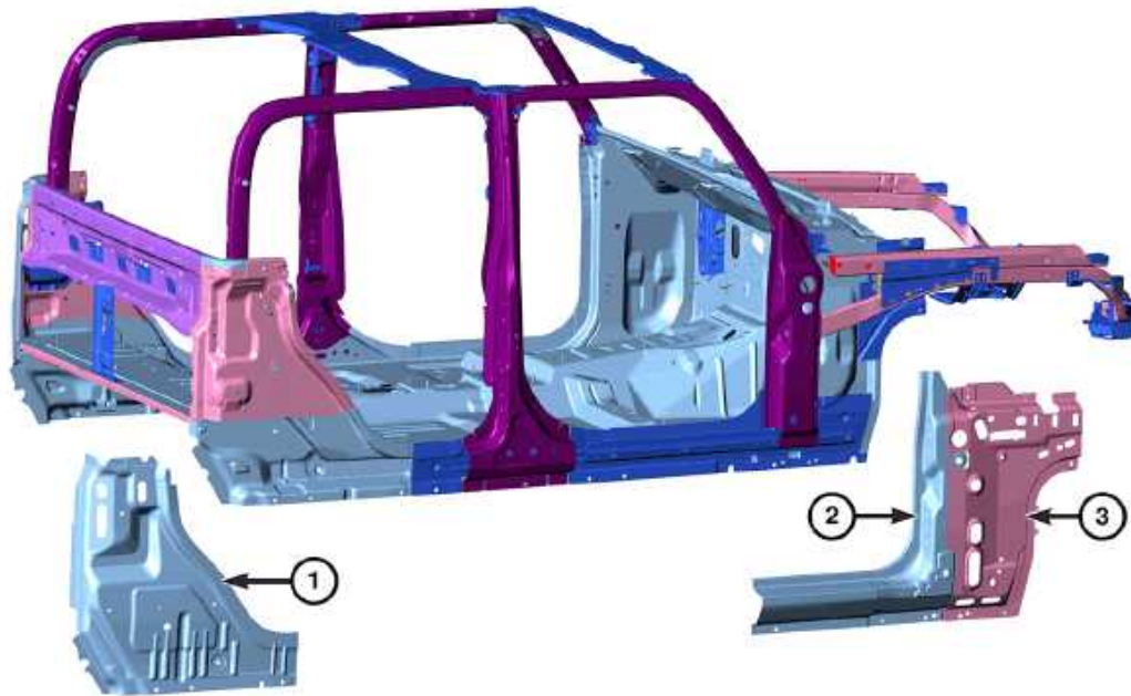
Fig. 9: Body In White (Right side view) Structure Identification Materials Courtesy of CHRYSLER GROUP, LLC
