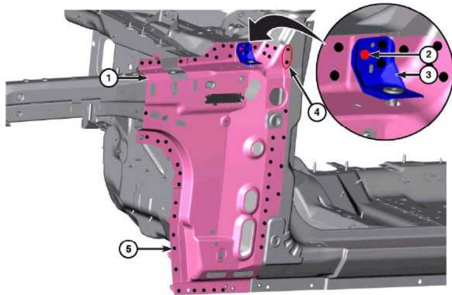
Fig. 2: Upper Load Path Beam Component Location
