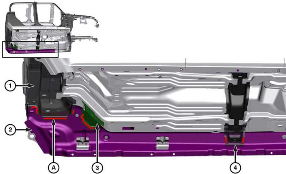
Fig. 41: Floor Crossmembers
