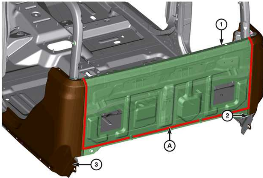
Fig. 47: Cab Back Panel
