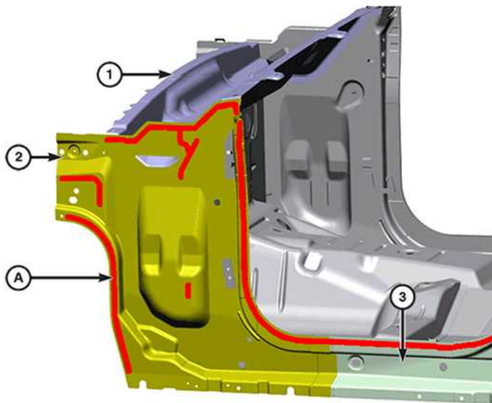
Fig. 21: Cowl Inner Side Panel
