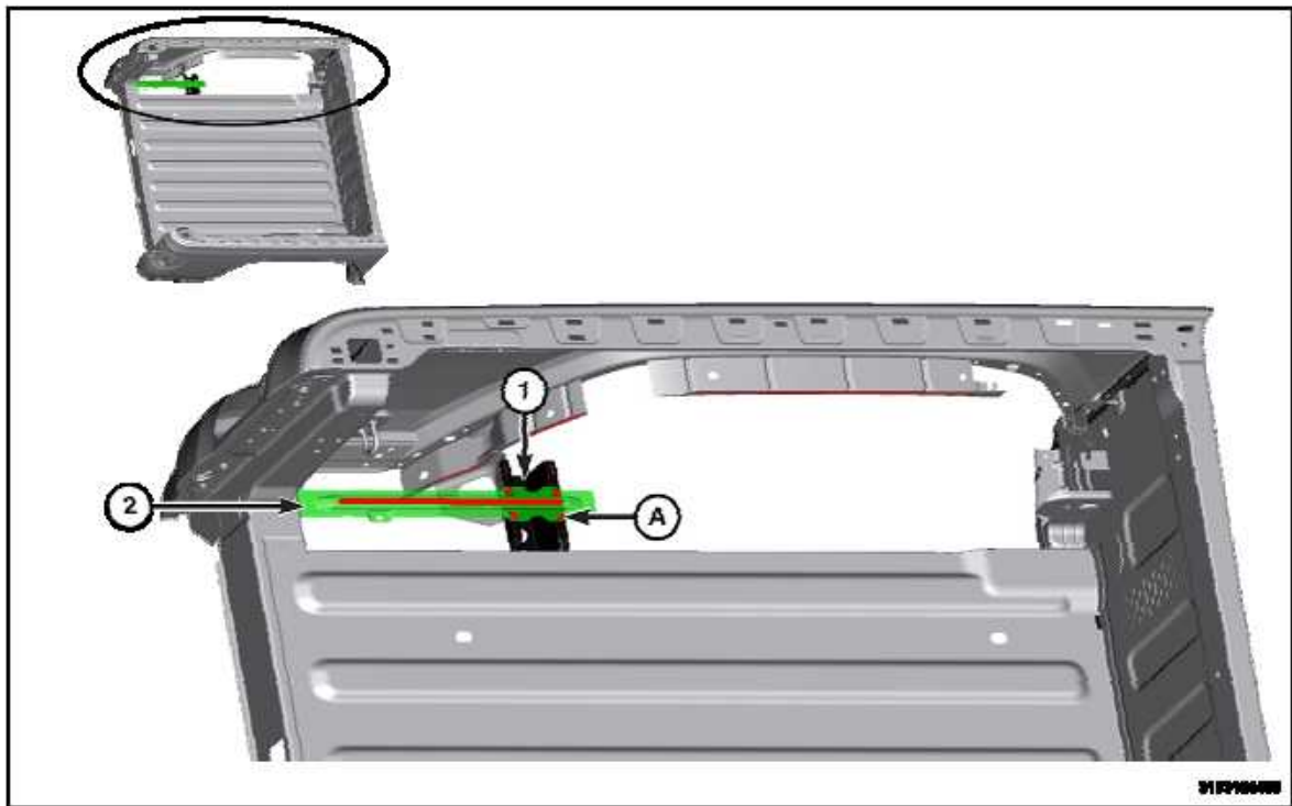
Fig. 53: Box Side Inner Reinforcement Courtesy of CHRYSLER GROUP, LLC
