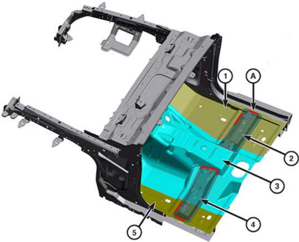
Fig. 28: Front Floor Courtesy of CHRYSLER GROUP, LLC
