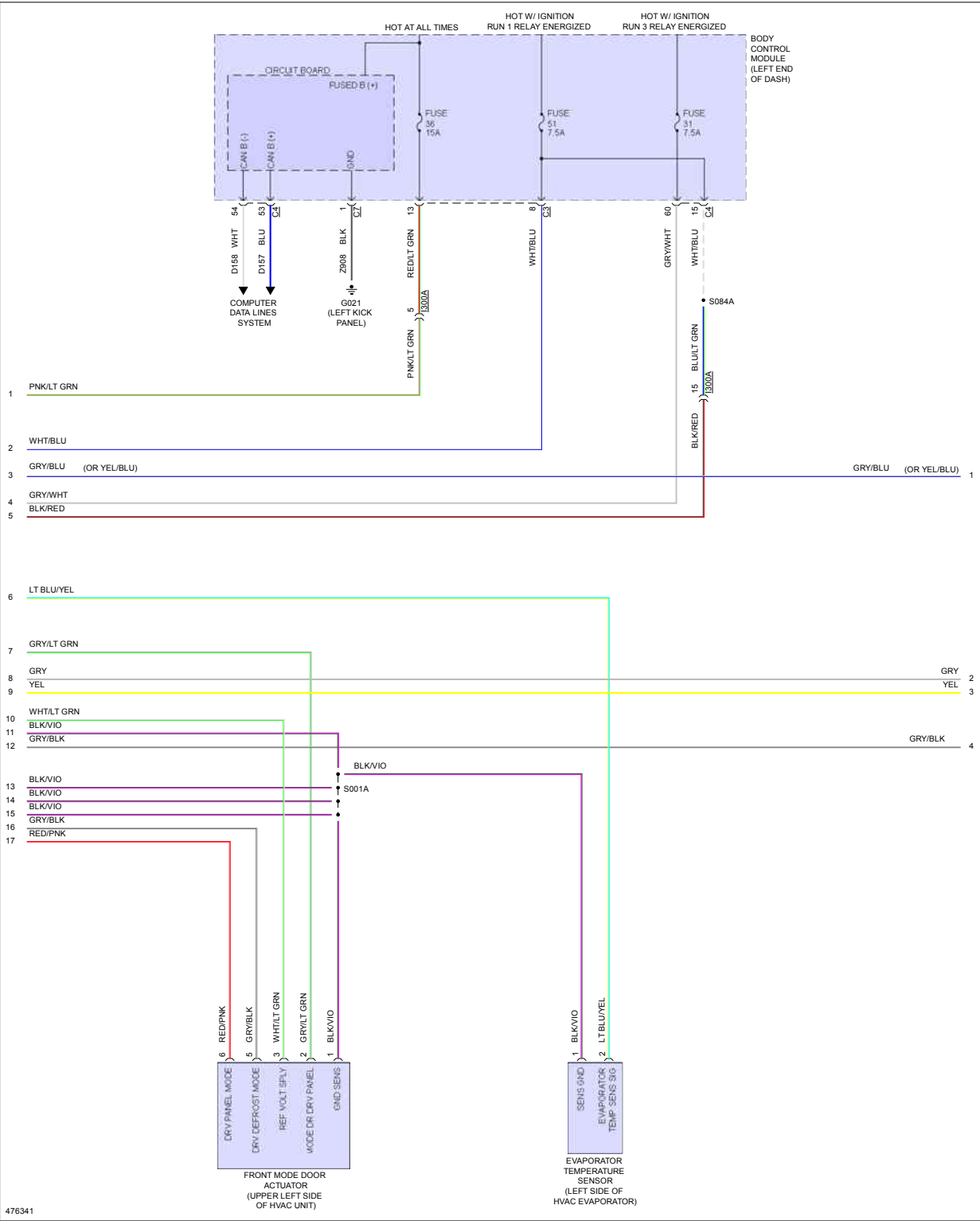
Fig 8: Manual A/C Circuit (3 of 5)
