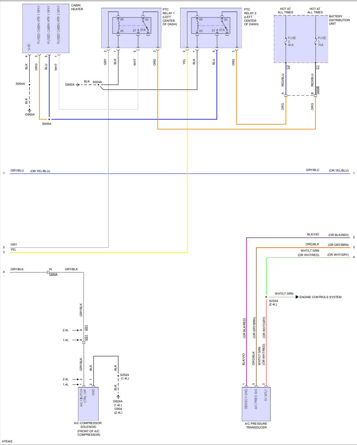
Fig 9: Manual A/C Circuit (4 of 5)
