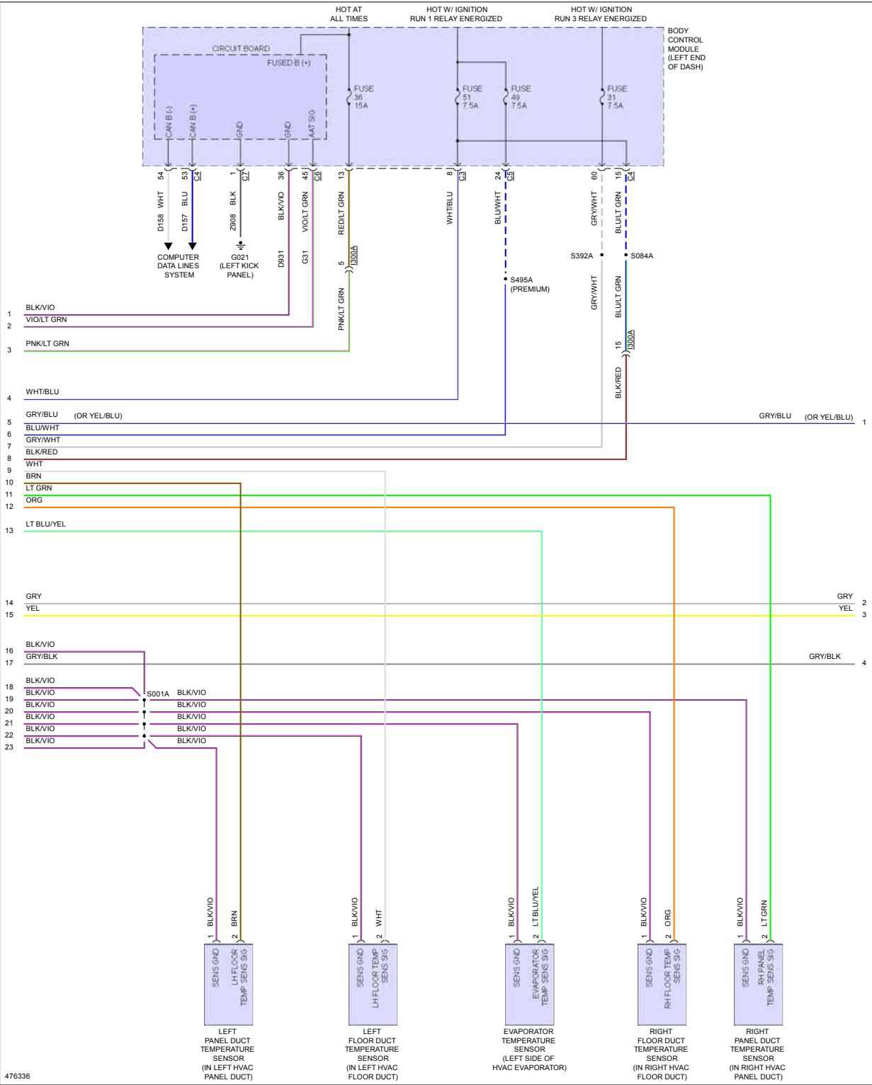
Fig 3: Automatic A/C Circuit (3 of 5)
