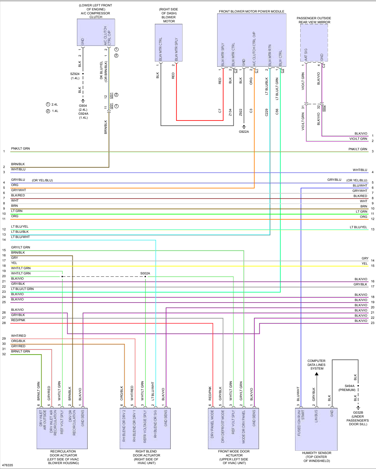
Fig 2: Automatic A/C Circuit (2 of 5)
