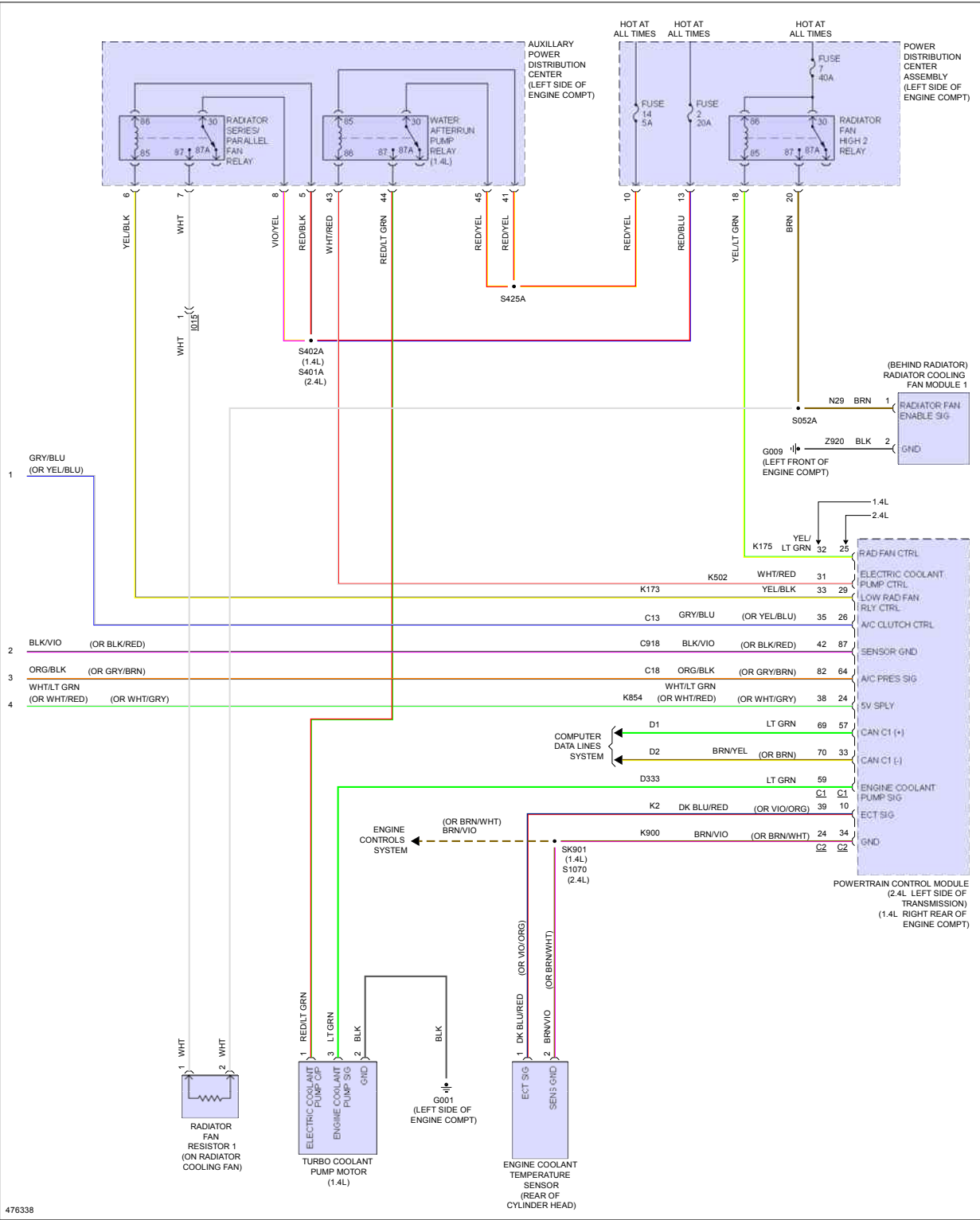
Fig 5: Automatic A/C Circuit (5 of 5)
