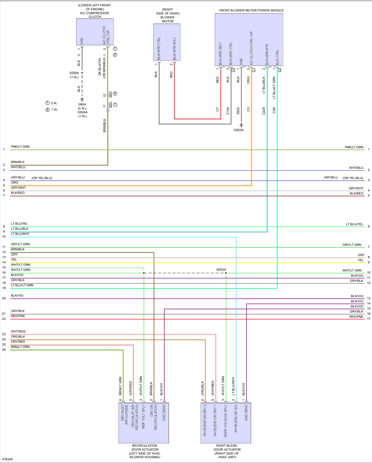
Fig 7: Manual A/C Circuit (2 of 5)
