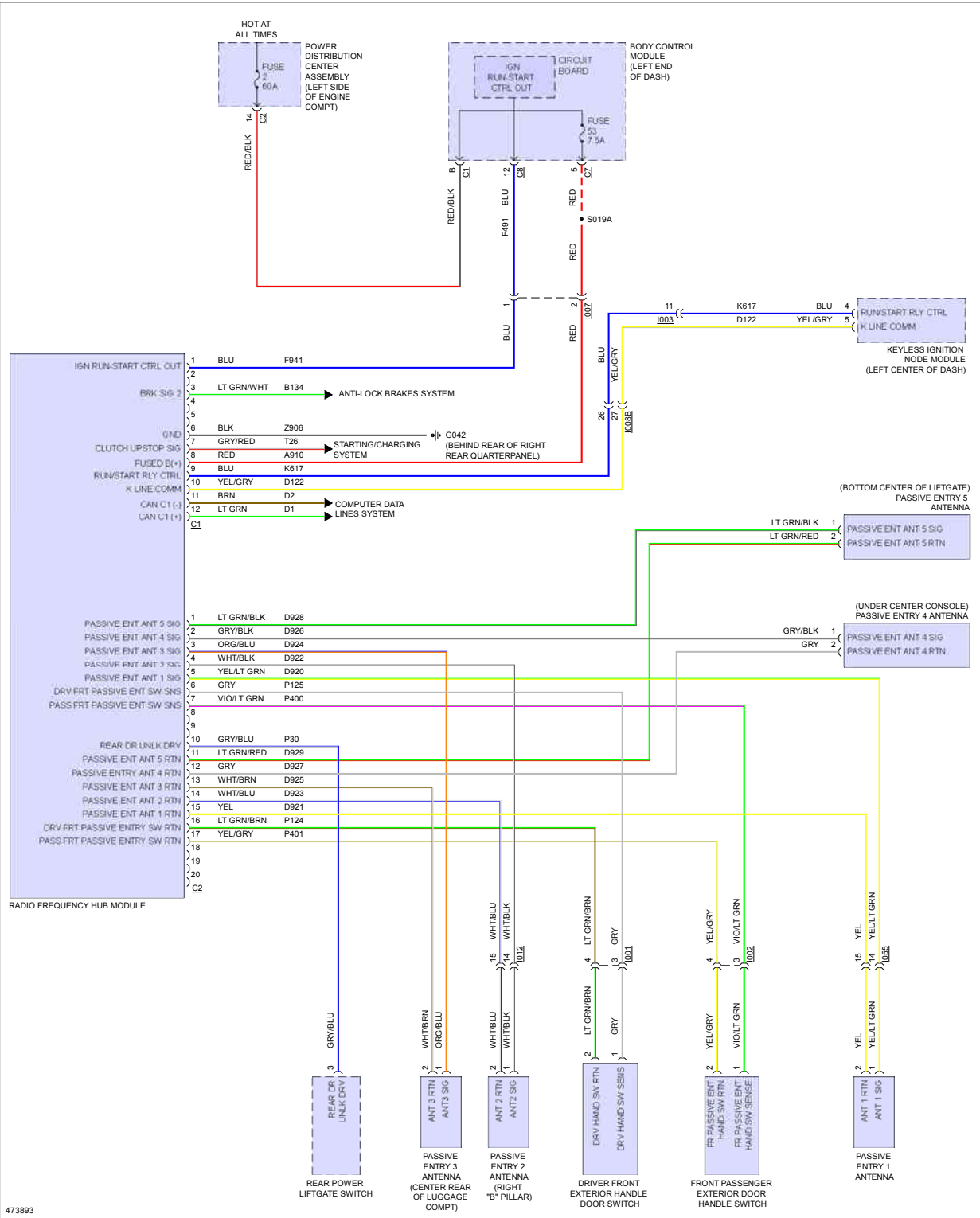
Fig 3: Passive Entry Circuit
