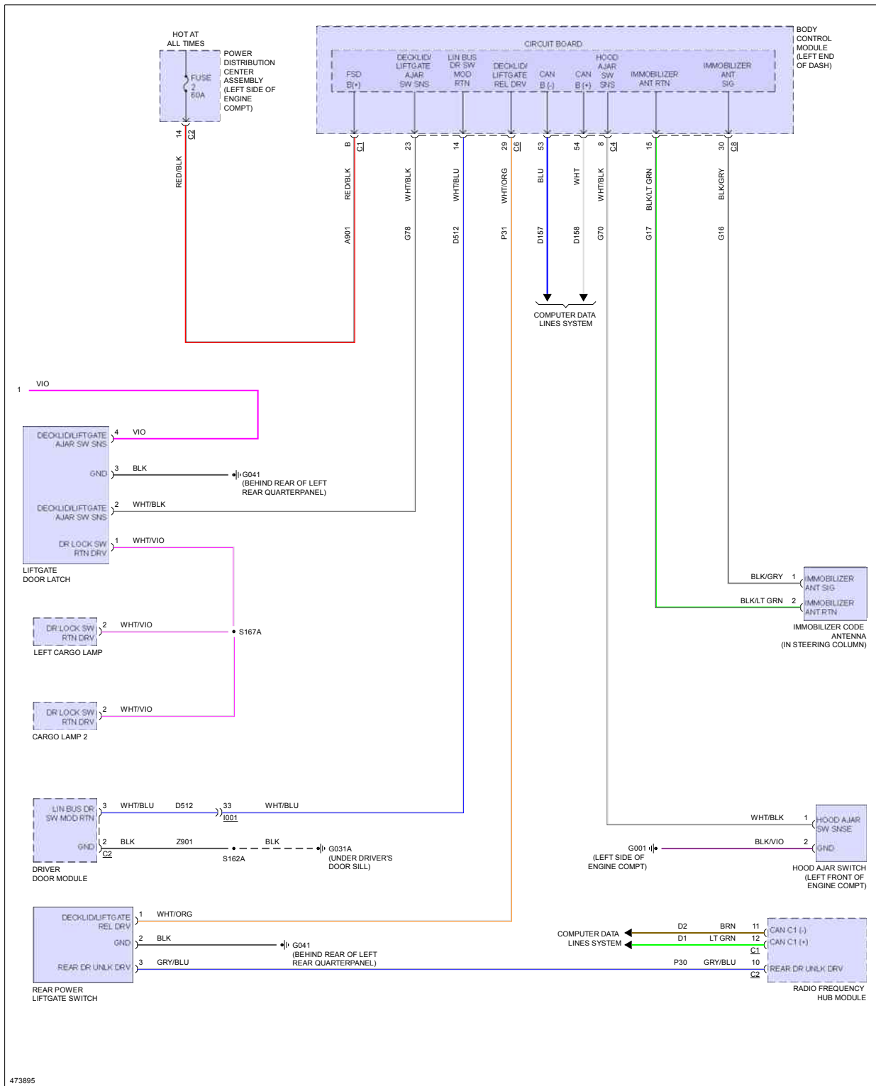
Fig 2: Forced Entry Circuit (2 of 2)
