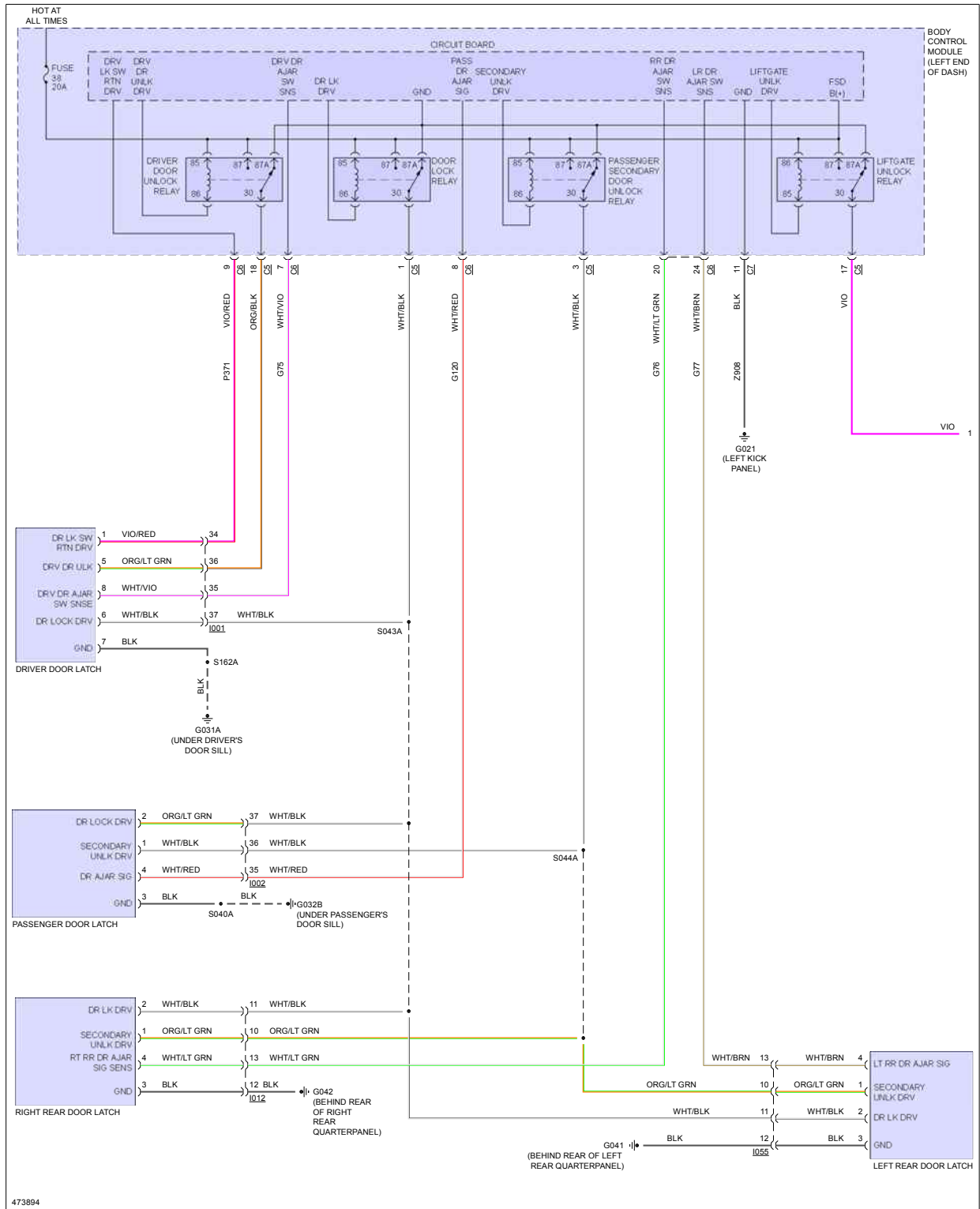
Fig 1: Forced Entry Circuit (1 of 2)
