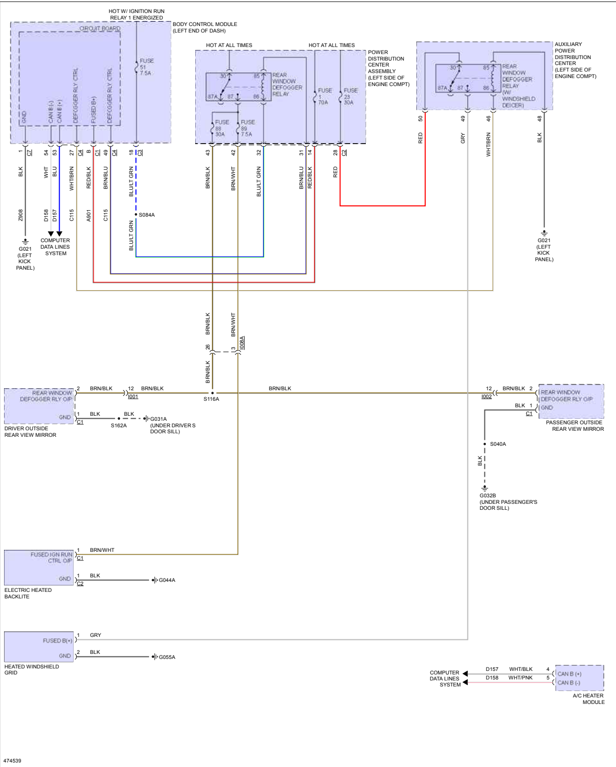
Fig 1: Defoggers Circuit
